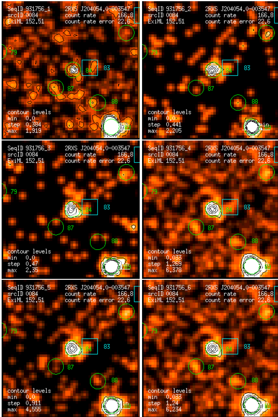
Figure 84: RASS 931756: detection 0084: band rate images, Gaussian filter: (1) PSPC channels 11 – 41, (2) 52 – 90, (3) 91 – 201, (4) 11 – 235, (5) 52 – 201, (6) 11 – 201. Broad band rates in counts/ks. Band rate contour levels in counts/ks/arcmin 2 .
