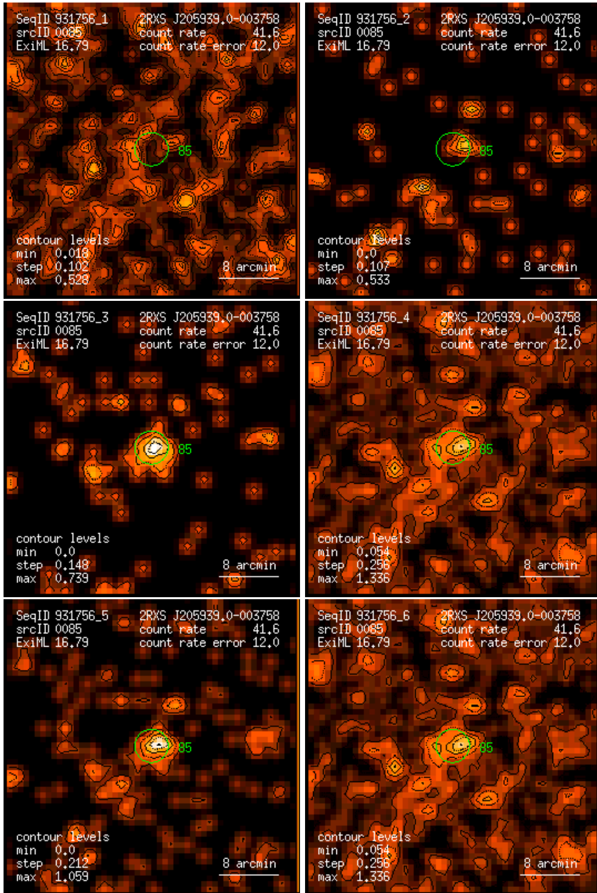
Figure 85: RASS 931756: detection 0085: band rate images, Gaussian filter: (1) PSPC channels 11 – 41, (2) 52 – 90, (3) 91 – 201, (4) 11 – 235, (5) 52 – 201, (6) 11 – 201. Broad band rates in counts/ks. Band rate contour levels in counts/ks/arcmin 2 .
