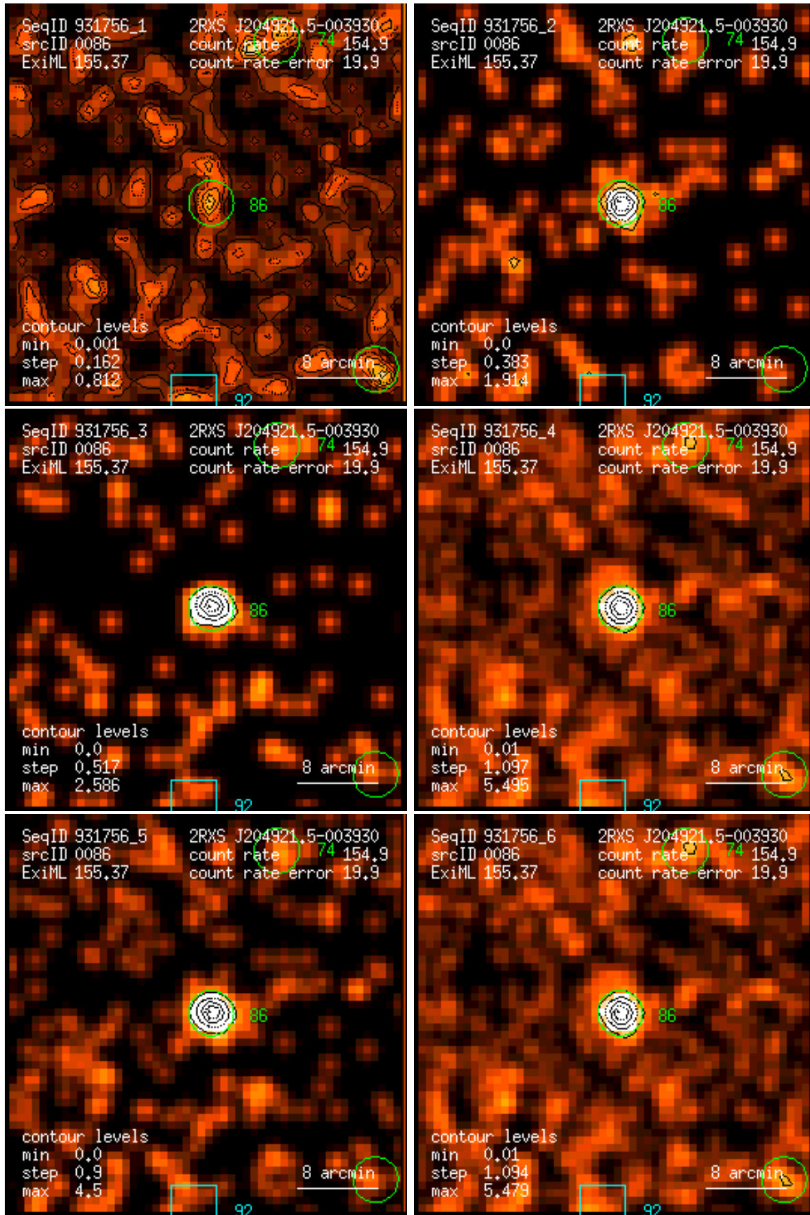
Figure 86: RASS 931756: detection 0086: band rate images, Gaussian filter: (1) PSPC channels 11 – 41, (2) 52 – 90, (3) 91 – 201, (4) 11 – 235, (5) 52 – 201, (6) 11 – 201. Broad band rates in counts/ks. Band rate contour levels in counts/ks/arcmin 2 .
