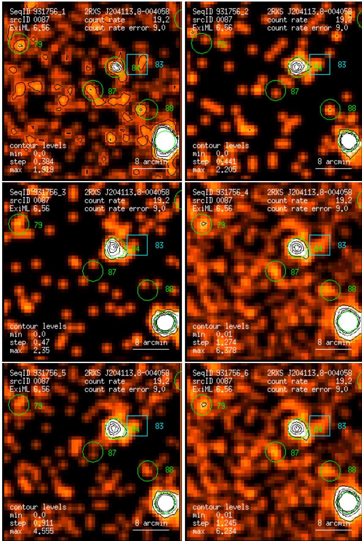
Figure 87: RASS 931756: detection 0087: band rate images, Gaussian filter: (1) PSPC channels 11 – 41, (2) 52 – 90, (3) 91 – 201, (4) 11 – 235, (5) 52 – 201, (6) 11 – 201. Broad band rates in counts/ks. Band rate contour levels in counts/ks/arcmin 2 .
