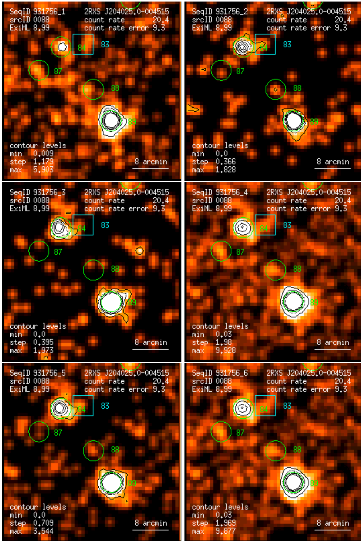
Figure 88: RASS 931756: detection 0088: band rate images, Gaussian filter: (1) PSPC channels 11 – 41, (2) 52 – 90, (3) 91 – 201, (4) 11 – 235, (5) 52 – 201, (6) 11 – 201. Broad band rates in counts/ks. Band rate contour levels in counts/ks/arcmin 2 .
