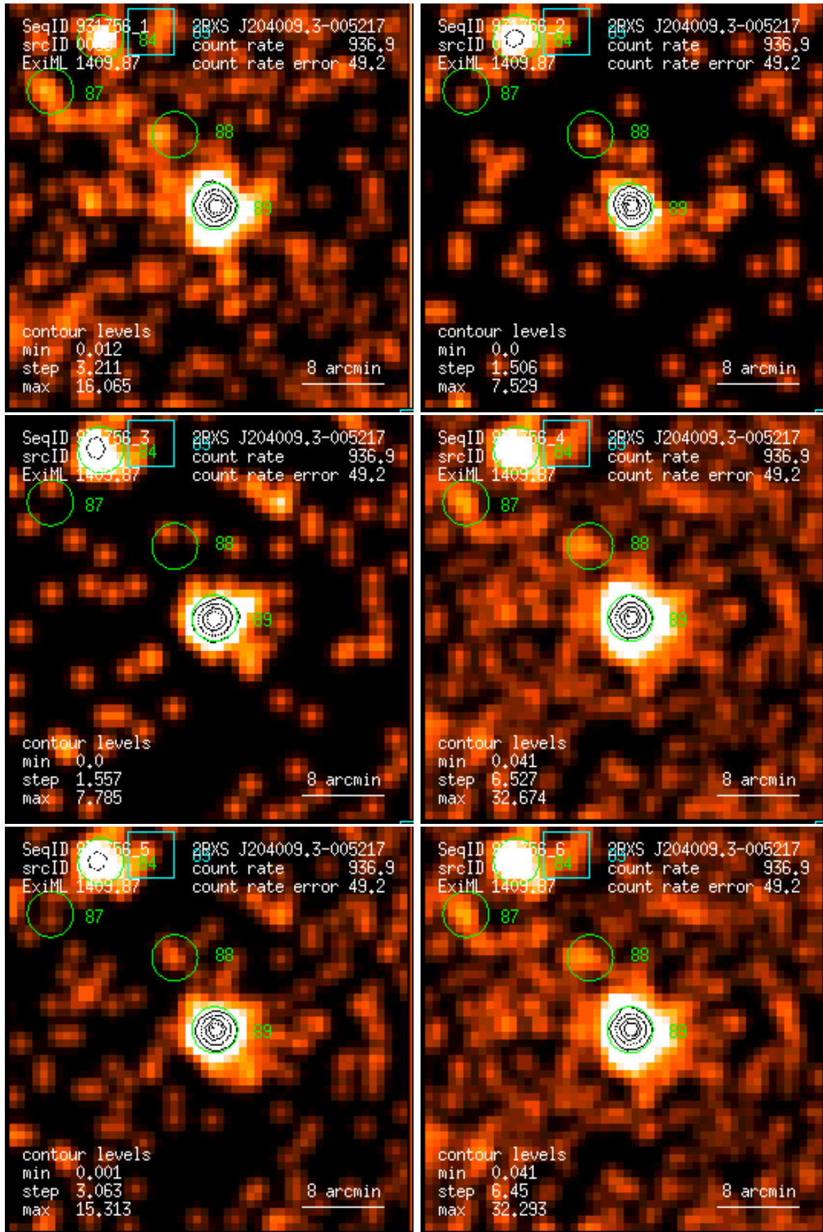
Figure 89: RASS 931756: detection 0089: band rate images, Gaussian filter: (1) PSPC channels 11 – 41, (2) 52 – 90, (3) 91 – 201, (4) 11 – 235, (5) 52 – 201, (6) 11 – 201. Broad band rates in counts/ks. Band rate contour levels in counts/ks/arcmin 2 .
