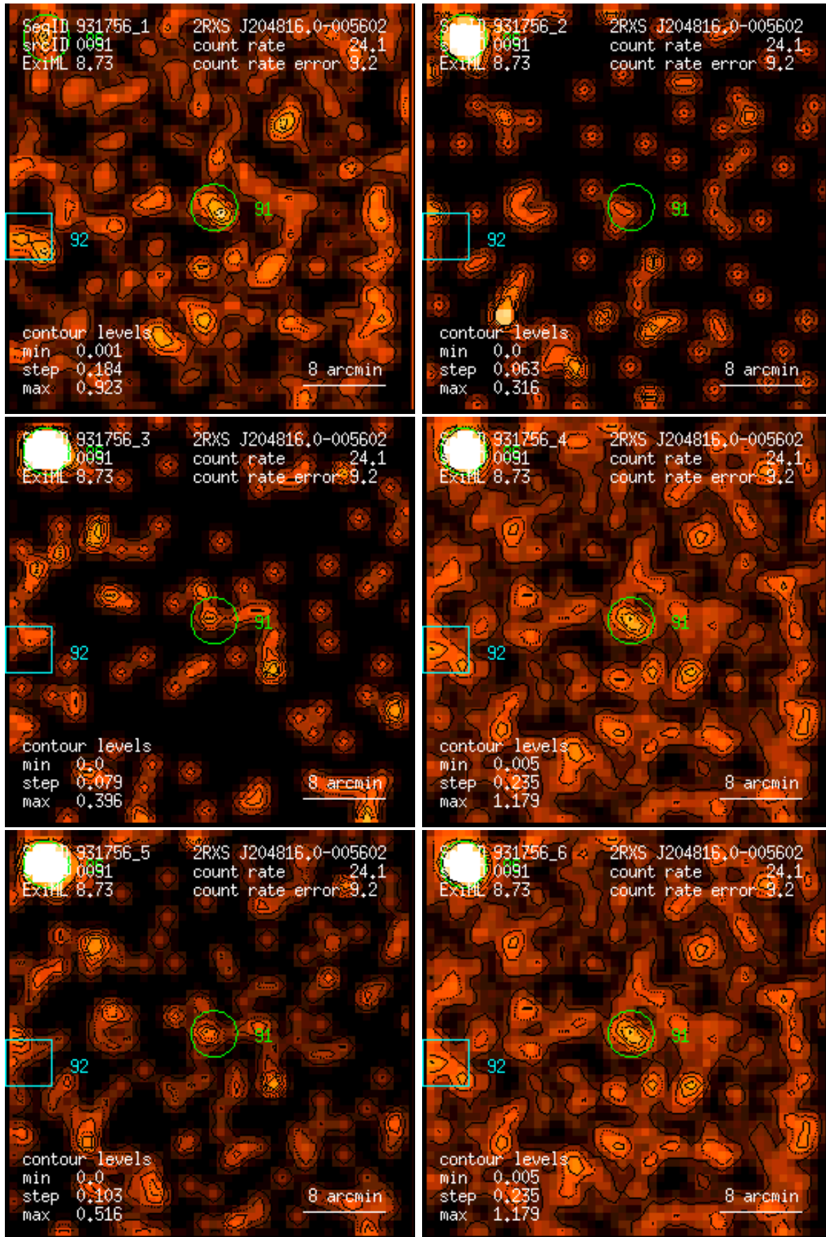
Figure 91: RASS 931756: detection 0091: band rate images, Gaussian filter: (1) PSPC channels 11 – 41, (2) 52 – 90, (3) 91 – 201, (4) 11 – 235, (5) 52 – 201, (6) 11 – 201. Broad band rates in counts/ks. Band rate contour levels in counts/ks/arcmin 2 .
