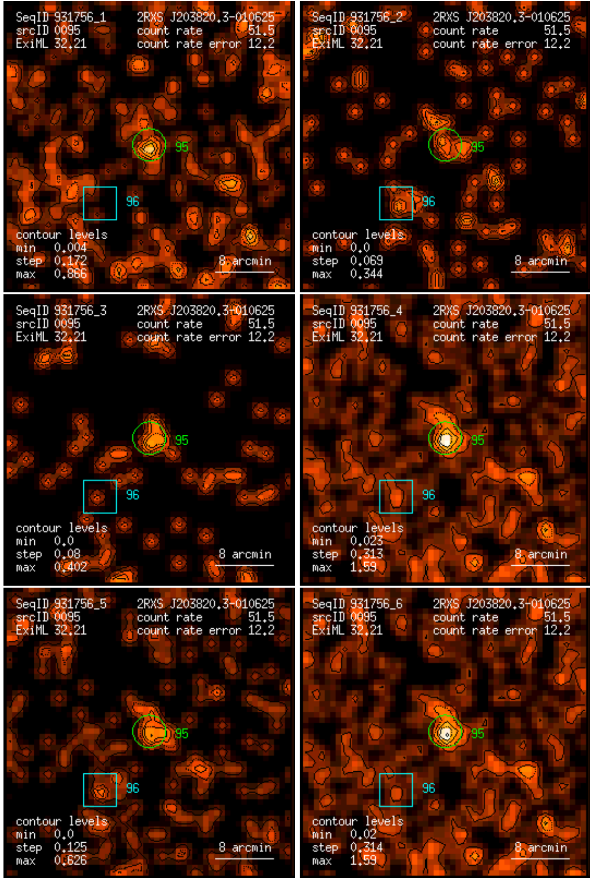
Figure 95: RASS 931756: detection 0095: band rate images, Gaussian filter: (1) PSPC channels 11 – 41, (2) 52 – 90, (3) 91 – 201, (4) 11 – 235, (5) 52 – 201, (6) 11 – 201. Broad band rates in counts/ks. Band rate contour levels in counts/ks/arcmin 2 .
