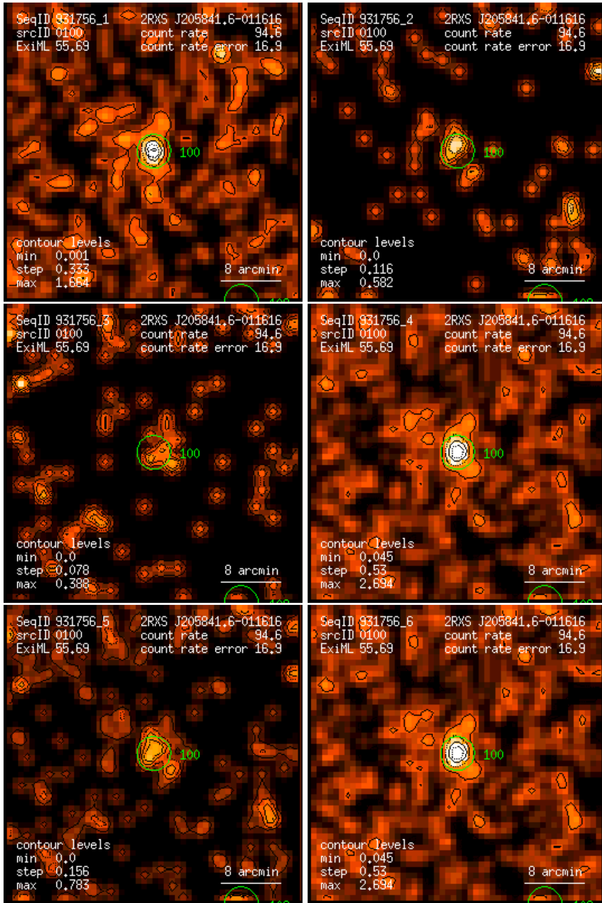
Figure 100: RASS 931756: detection 0100: band rate images, Gaussian filter: (1) PSPC channels 11 – 41, (2) 52 – 90, (3) 91 – 201, (4) 11 – 235, (5) 52 – 201, (6) 11 – 201. Broad band rates in counts/ks. Band rate contour levels in counts/ks/arcmin 2 .
