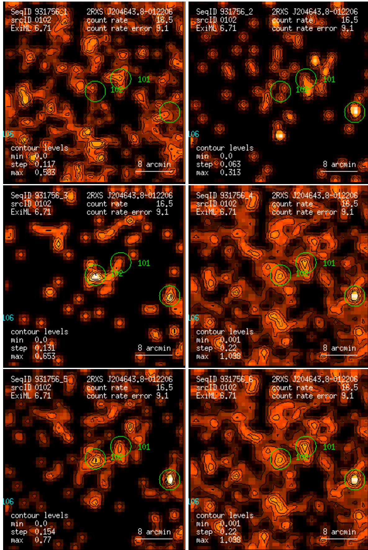
Figure 102: RASS 931756: detection 0102: band rate images, Gaussian filter: (1) PSPC channels 11 – 41, (2) 52 – 90, (3) 91 – 201, (4) 11 – 235, (5) 52 – 201, (6) 11 – 201. Broad band rates in counts/ks. Band rate contour levels in counts/ks/arcmin 2 .
