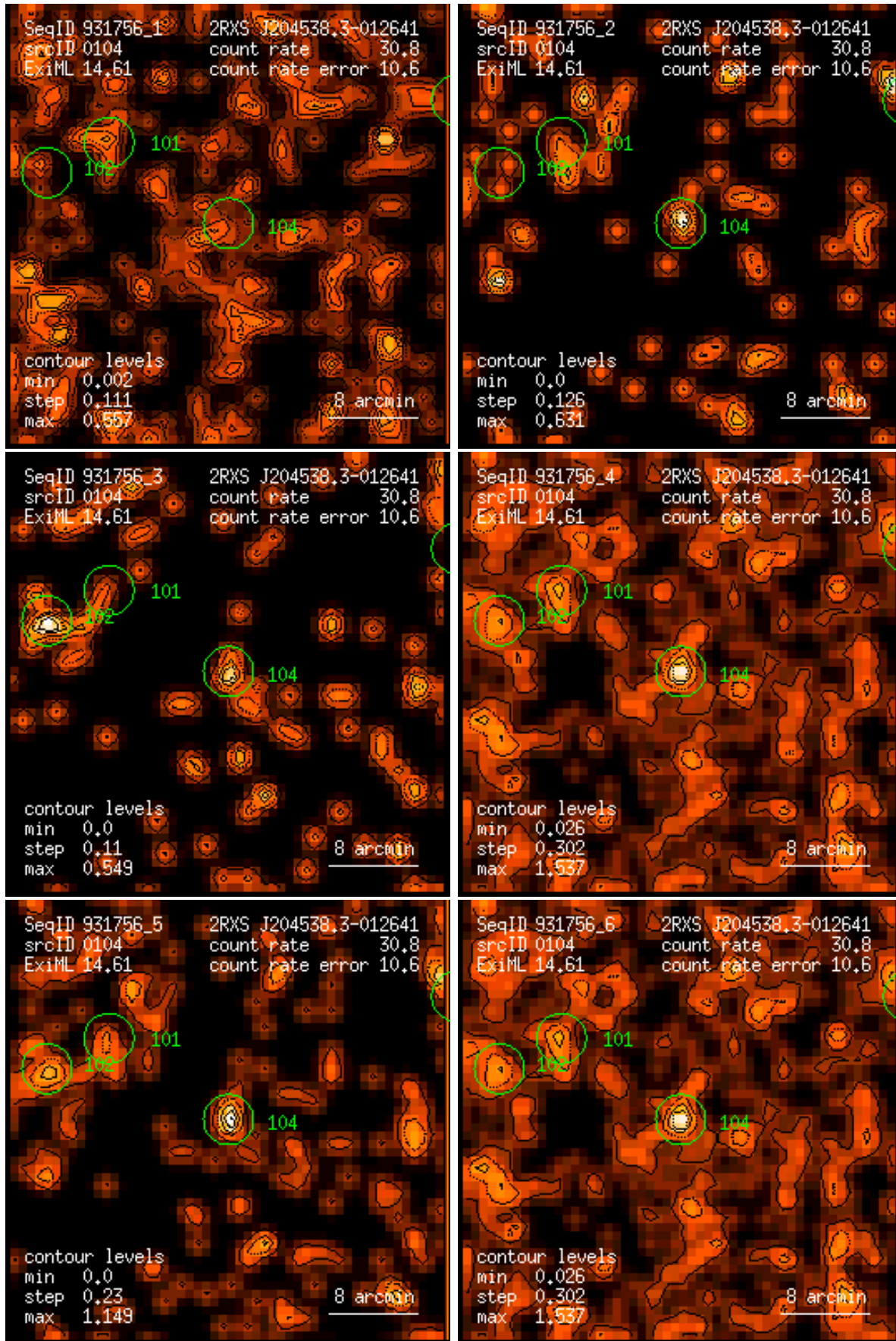
Figure 104: RASS 931756: detection 0104: band rate images, Gaussian filter: (1) PSPC channels 11 – 41, (2) 52 – 90, (3) 91 – 201, (4) 11 – 235, (5) 52 – 201, (6) 11 – 201. Broad band rates in counts/ks. Band rate contour levels in counts/ks/arcmin 2 .
