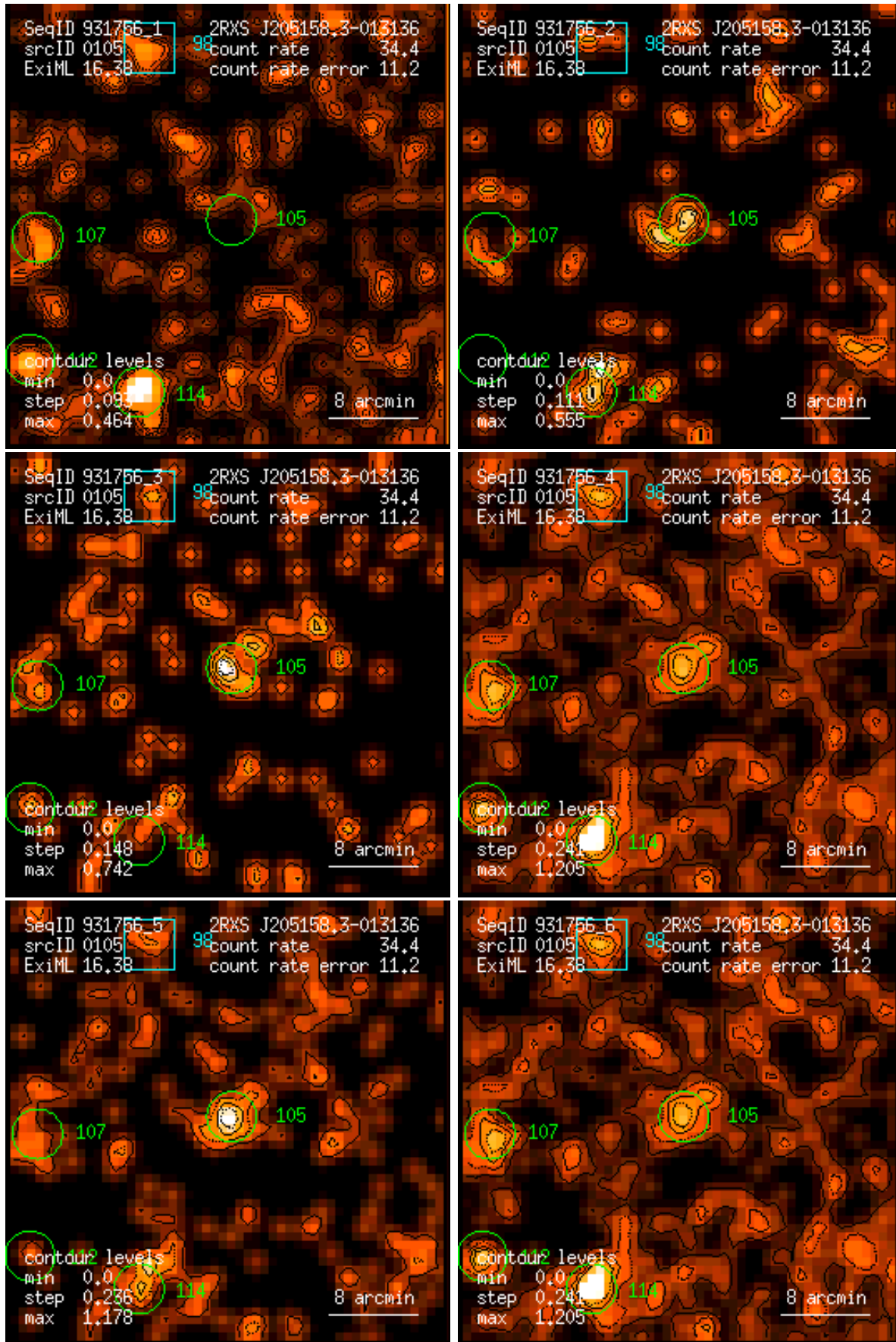
Figure 105: RASS 931756: detection 0105: band rate images, Gaussian filter: (1) PSPC channels 11 – 41, (2) 52 – 90, (3) 91 – 201, (4) 11 – 235, (5) 52 – 201, (6) 11 – 201. Broad band rates in counts/ks. Band rate contour levels in counts/ks/arcmin 2 .
