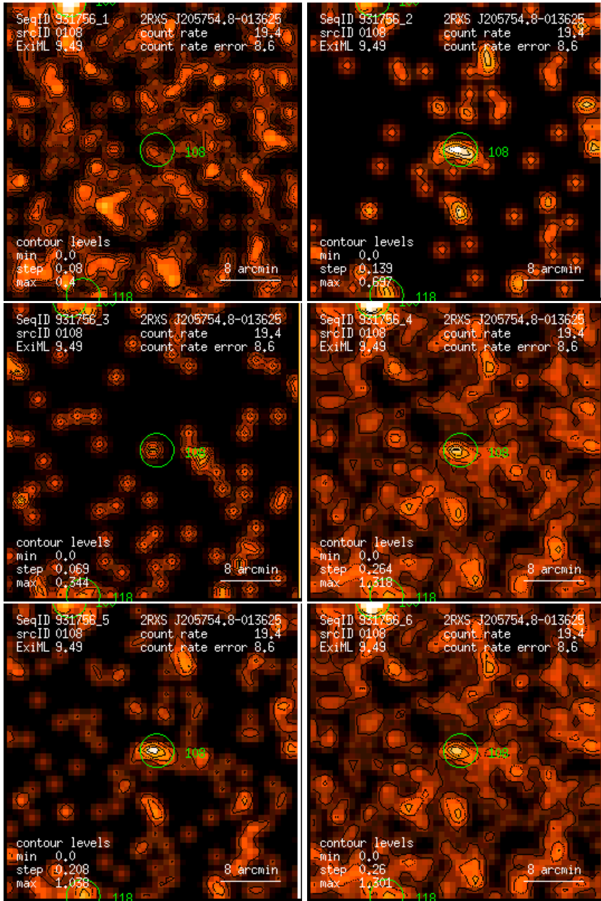
Figure 108: RASS 931756: detection 0108: band rate images, Gaussian filter: (1) PSPC channels 11 – 41, (2) 52 – 90, (3) 91 – 201, (4) 11 – 235, (5) 52 – 201, (6) 11 – 201. Broad band rates in counts/ks. Band rate contour levels in counts/ks/arcmin 2 .
