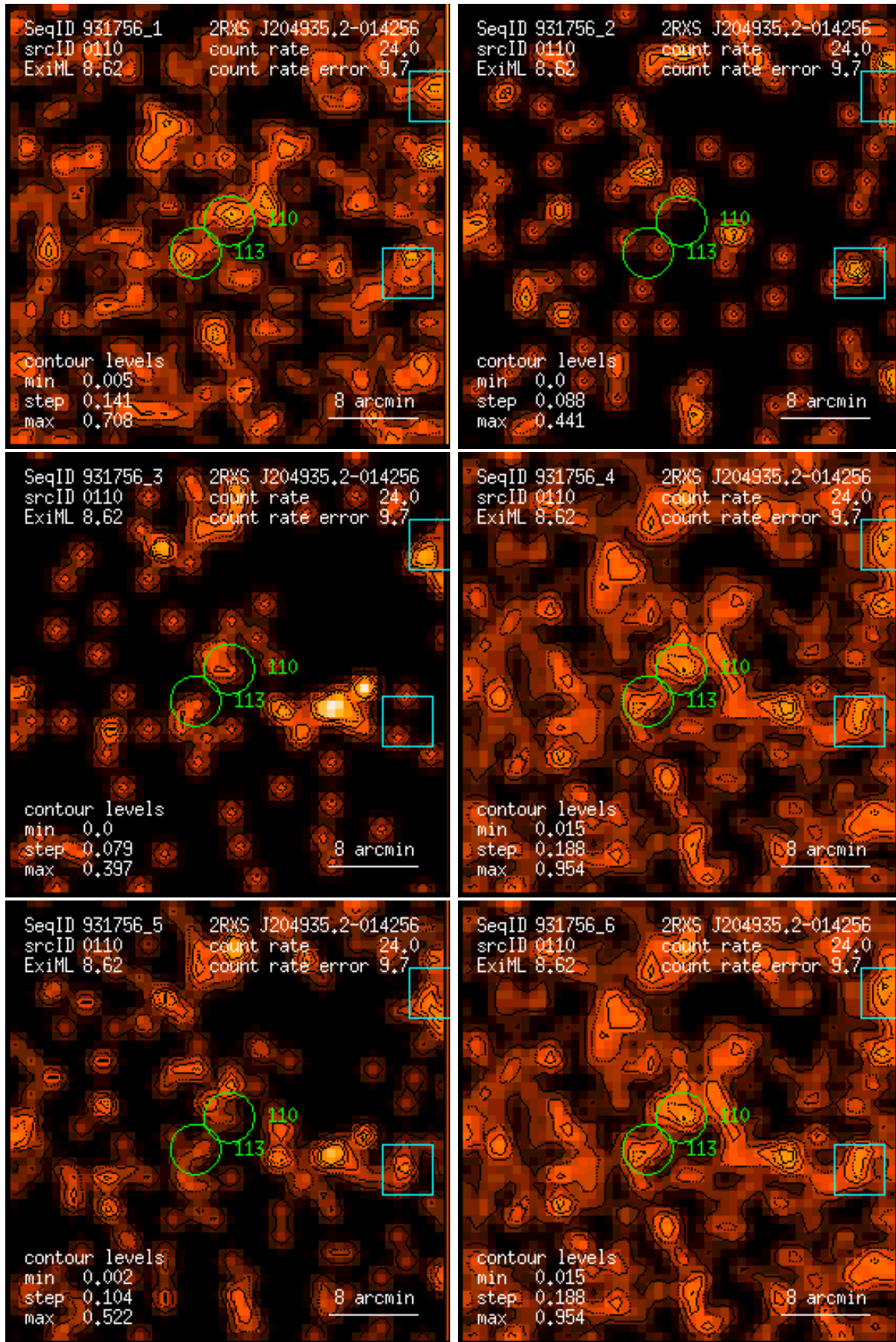
Figure 110: RASS 931756: detection 0110: band rate images, Gaussian filter: (1) PSPC channels 11 – 41, (2) 52 – 90, (3) 91 – 201, (4) 11 – 235, (5) 52 – 201, (6) 11 – 201. Broad band rates in counts/ks. Band rate contour levels in counts/ks/arcmin 2 .
