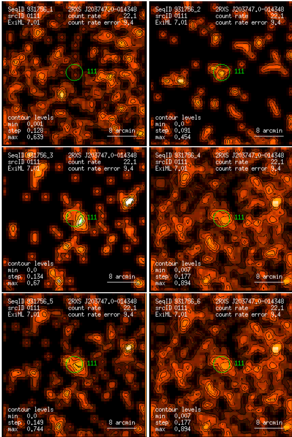
Figure 111: RASS 931756: detection 0111: band rate images, Gaussian filter: (1) PSPC channels 11 – 41, (2) 52 – 90, (3) 91 – 201, (4) 11 – 235, (5) 52 – 201, (6) 11 – 201. Broad band rates in counts/ks. Band rate contour levels in counts/ks/arcmin 2 .
