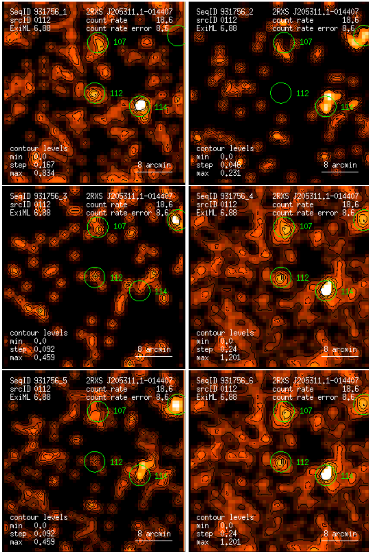
Figure 112: RASS 931756: detection 0112: band rate images, Gaussian filter: (1) PSPC channels 11 – 41, (2) 52 – 90, (3) 91 – 201, (4) 11 – 235, (5) 52 – 201, (6) 11 – 201. Broad band rates in counts/ks. Band rate contour levels in counts/ks/arcmin 2 .
