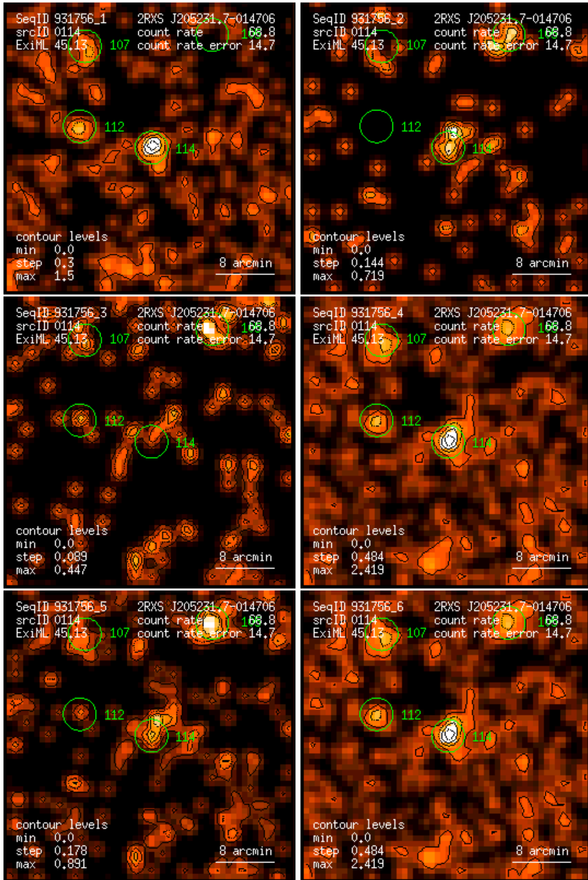
Figure 114: RASS 931756: detection 0114: band rate images, Gaussian filter: (1) PSPC channels 11 – 41, (2) 52 – 90, (3) 91 – 201, (4) 11 – 235, (5) 52 – 201, (6) 11 – 201. Broad band rates in counts/ks. Band rate contour levels in counts/ks/arcmin 2 .
