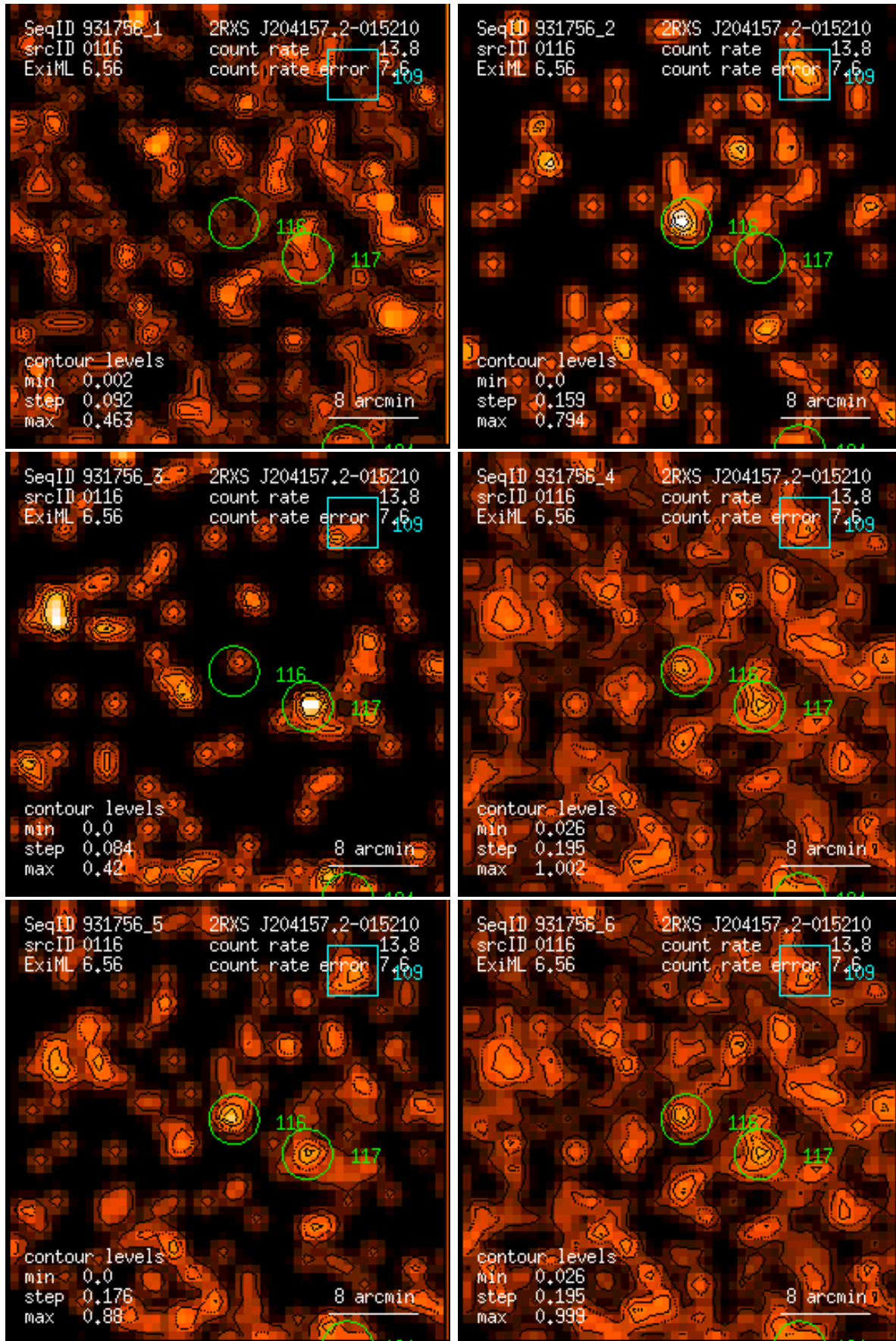
Figure 116: RASS 931756: detection 0116: band rate images, Gaussian filter: (1) PSPC channels 11 – 41, (2) 52 – 90, (3) 91 – 201, (4) 11 – 235, (5) 52 – 201, (6) 11 – 201. Broad band rates in counts/ks. Band rate contour levels in counts/ks/arcmin 2 .
