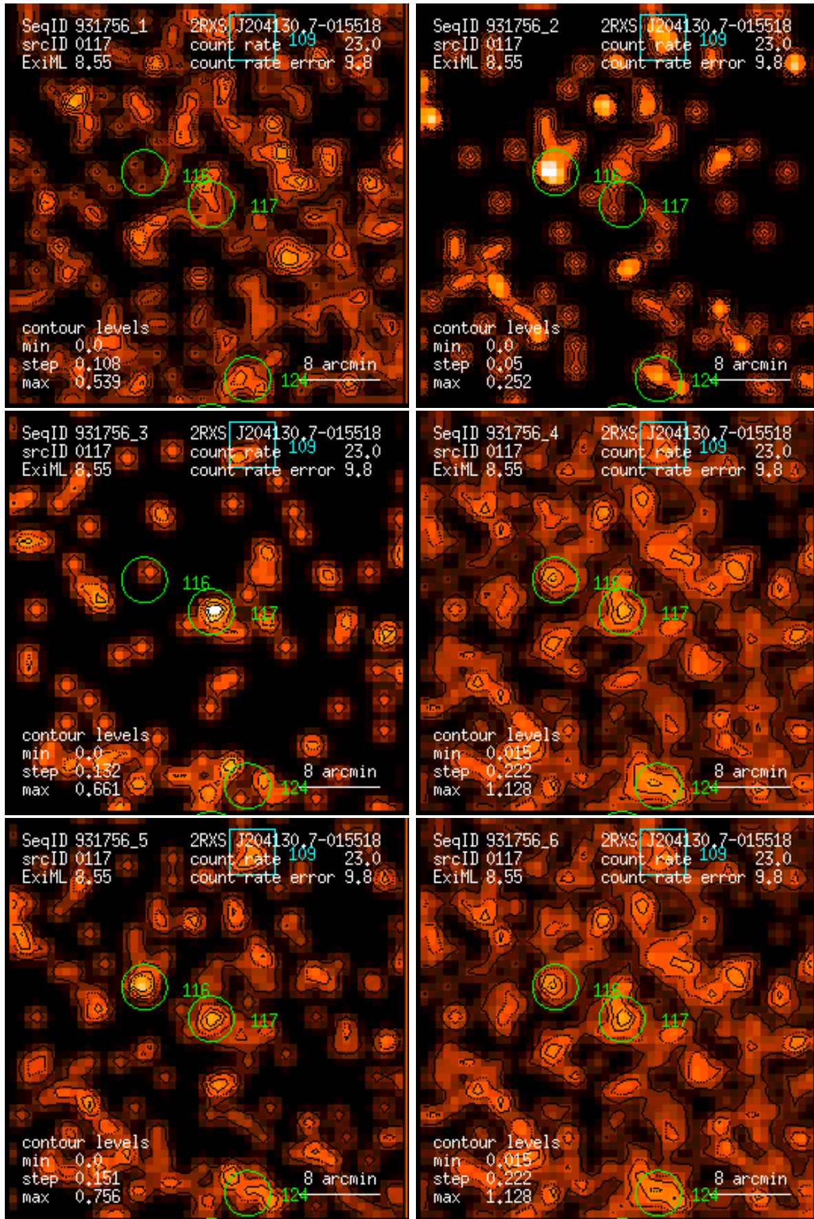
Figure 117: RASS 931756: detection 0117: band rate images, Gaussian filter: (1) PSPC channels 11 – 41, (2) 52 – 90, (3) 91 – 201, (4) 11 – 235, (5) 52 – 201, (6) 11 – 201. Broad band rates in counts/ks. Band rate contour levels in counts/ks/arcmin 2 .
