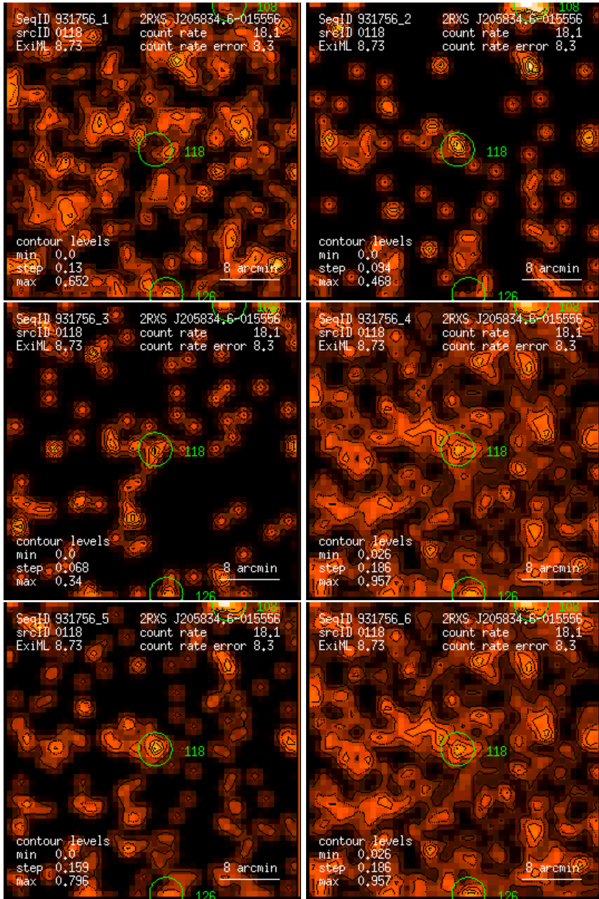
Figure 118: RASS 931756: detection 0118: band rate images, Gaussian filter: (1) PSPC channels 11 – 41, (2) 52 – 90, (3) 91 – 201, (4) 11 – 235, (5) 52 – 201, (6) 11 – 201. Broad band rates in counts/ks. Band rate contour levels in counts/ks/arcmin 2 .
