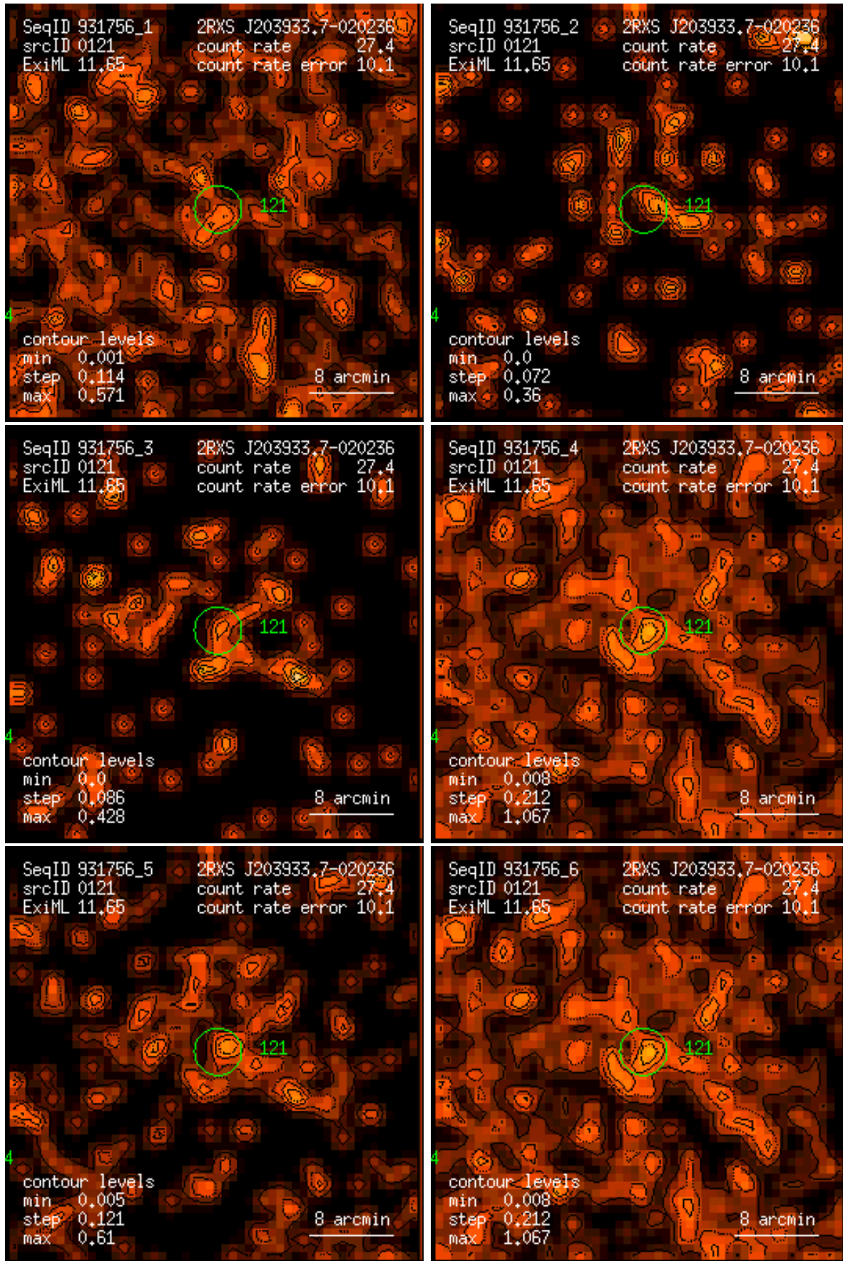
Figure 121: RASS 931756: detection 0121: band rate images, Gaussian filter: (1) PSPC channels 11 – 41, (2) 52 – 90, (3) 91 – 201, (4) 11 – 235, (5) 52 – 201, (6) 11 – 201. Broad band rates in counts/ks. Band rate contour levels in counts/ks/arcmin 2 .
