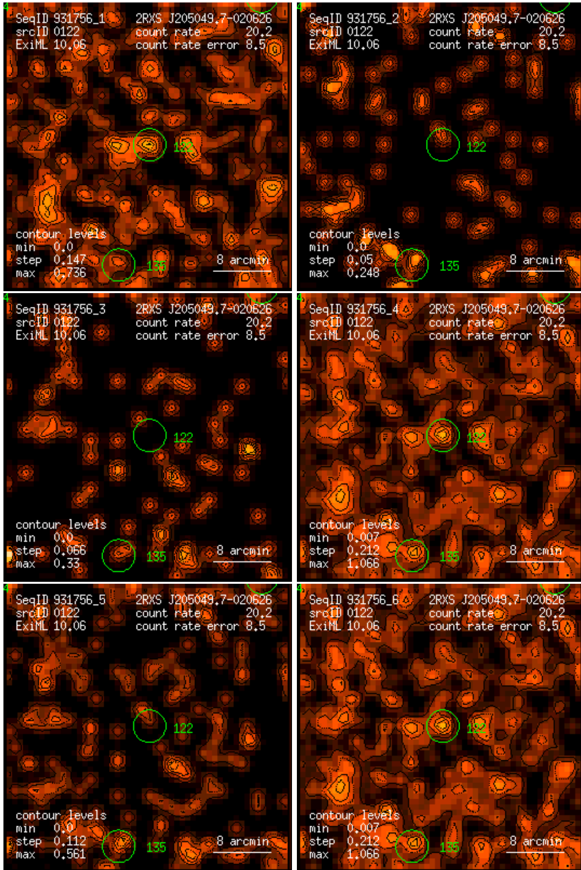
Figure 122: RASS 931756: detection 0122: band rate images, Gaussian filter: (1) PSPC channels 11 – 41, (2) 52 – 90, (3) 91 – 201, (4) 11 – 235, (5) 52 – 201, (6) 11 – 201. Broad band rates in counts/ks. Band rate contour levels in counts/ks/arcmin 2 .
