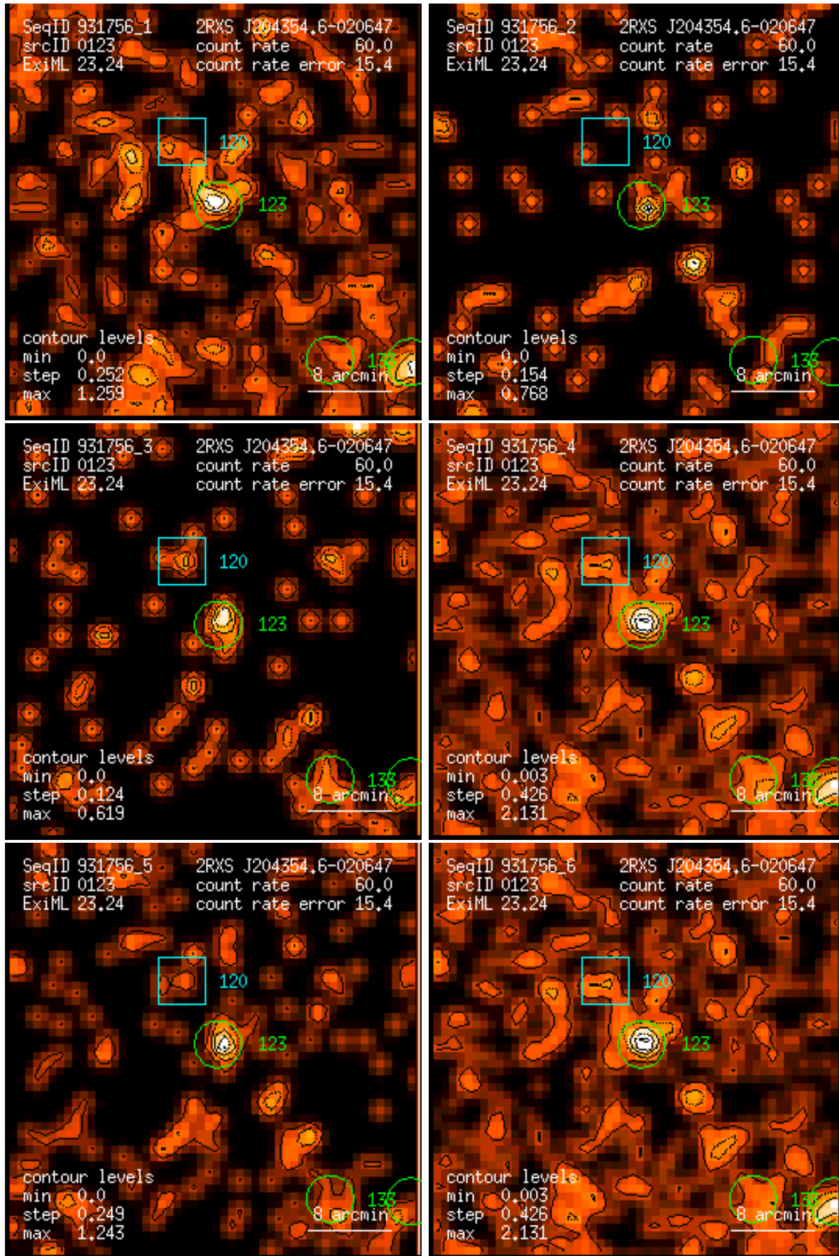
Figure 123: RASS 931756: detection 0123: band rate images, Gaussian filter: (1) PSPC channels 11 – 41, (2) 52 – 90, (3) 91 – 201, (4) 11 – 235, (5) 52 – 201, (6) 11 – 201. Broad band rates in counts/ks. Band rate contour levels in counts/ks/arcmin 2 .
