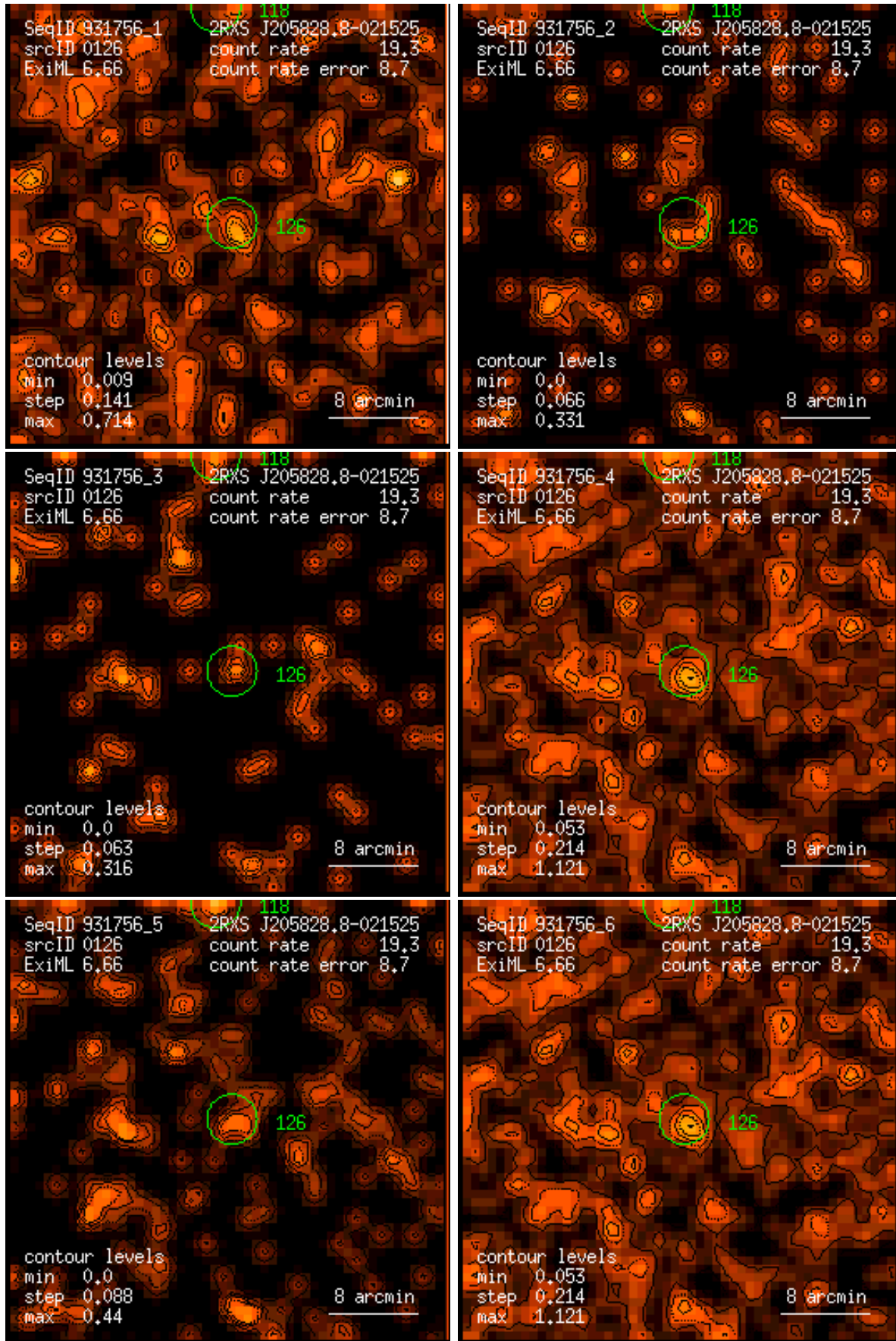
Figure 126: RASS 931756: detection 0126: band rate images, Gaussian filter: (1) PSPC channels 11 – 41, (2) 52 – 90, (3) 91 – 201, (4) 11 – 235, (5) 52 – 201, (6) 11 – 201. Broad band rates in counts/ks. Band rate contour levels in counts/ks/arcmin 2 .
