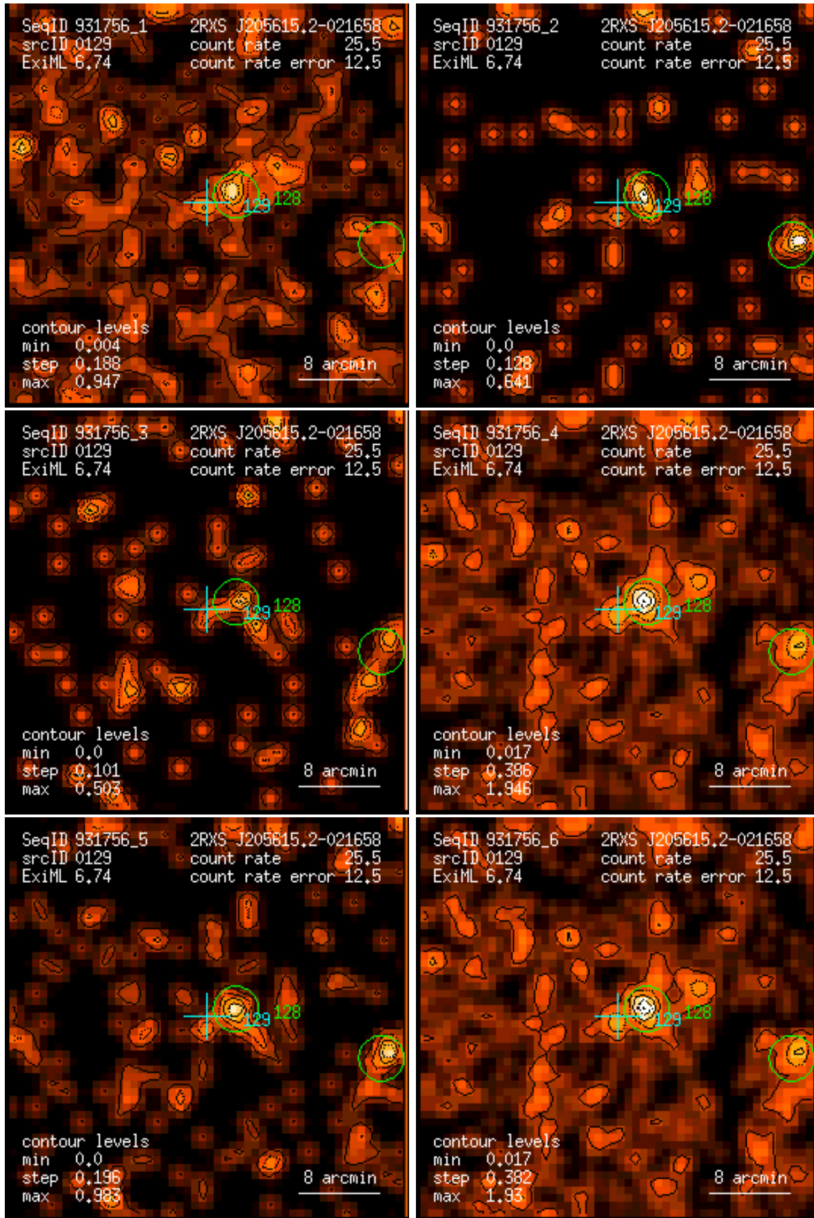
Figure 129: RASS 931756: detection 0129: band rate images, Gaussian filter: (1) PSPC channels 11 – 41, (2) 52 – 90, (3) 91 – 201, (4) 11 – 235, (5) 52 – 201, (6) 11 – 201. Broad band rates in counts/ks. Band rate contour levels in counts/ks/arcmin 2 .
