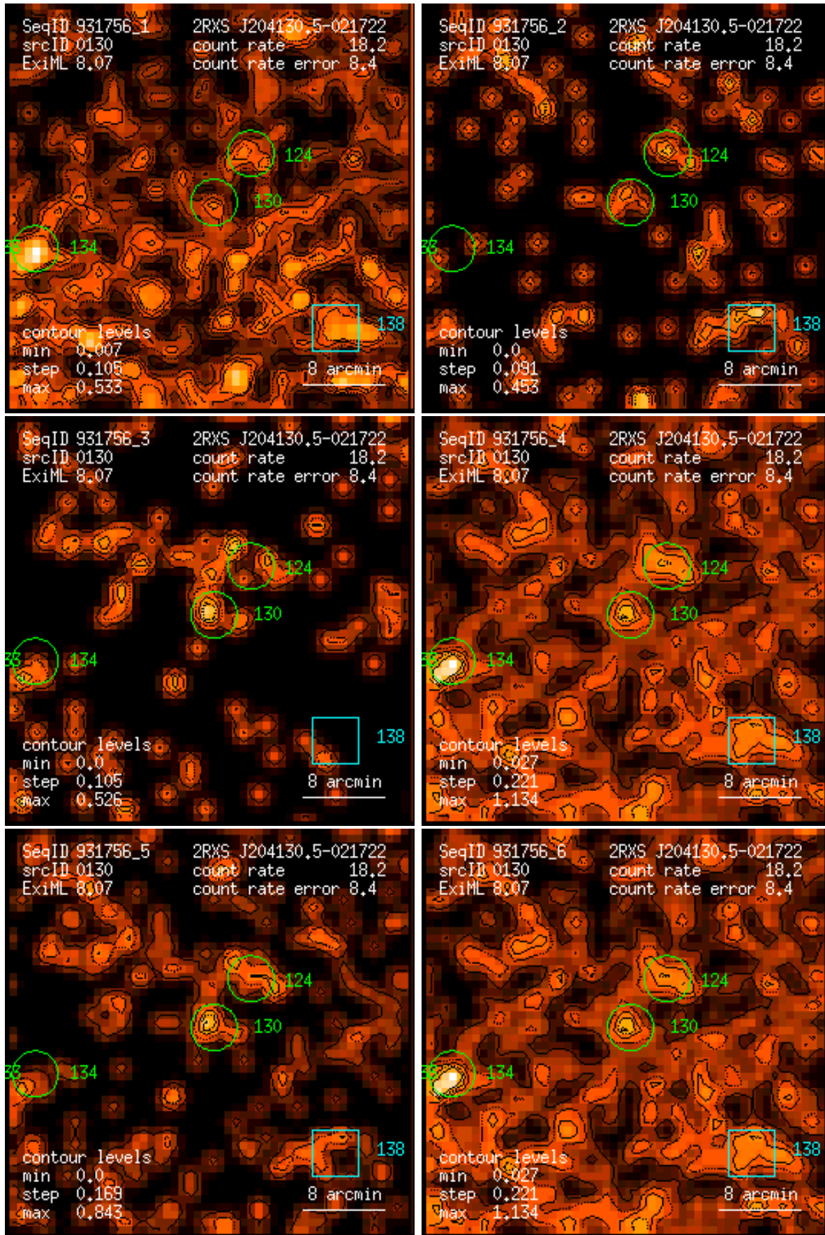
Figure 130: RASS 931756: detection 0130: band rate images, Gaussian filter: (1) PSPC channels 11 – 41, (2) 52 – 90, (3) 91 – 201, (4) 11 – 235, (5) 52 – 201, (6) 11 – 201. Broad band rates in counts/ks. Band rate contour levels in counts/ks/arcmin 2 .
