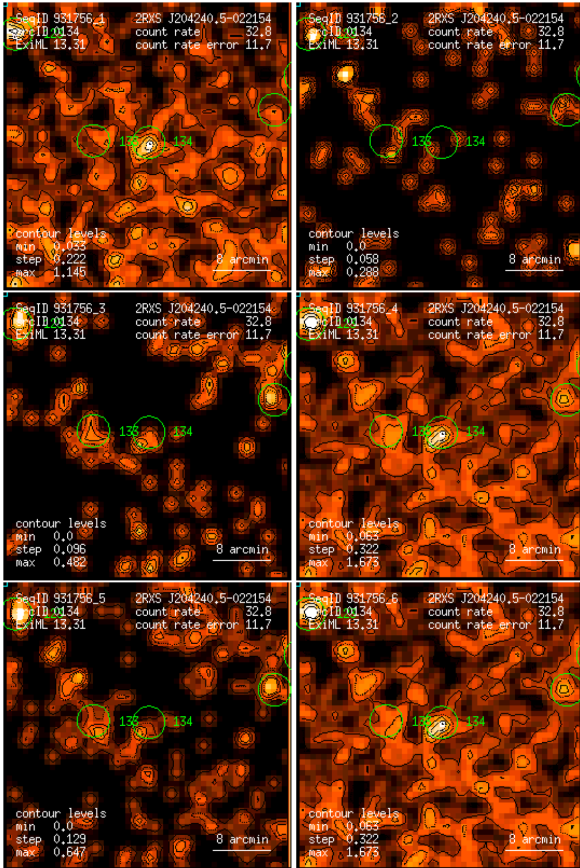
Figure 134: RASS 931756: detection 0134: band rate images, Gaussian filter: (1) PSPC channels 11 – 41, (2) 52 – 90, (3) 91 – 201, (4) 11 – 235, (5) 52 – 201, (6) 11 – 201. Broad band rates in counts/ks. Band rate contour levels in counts/ks/arcmin 2 .
