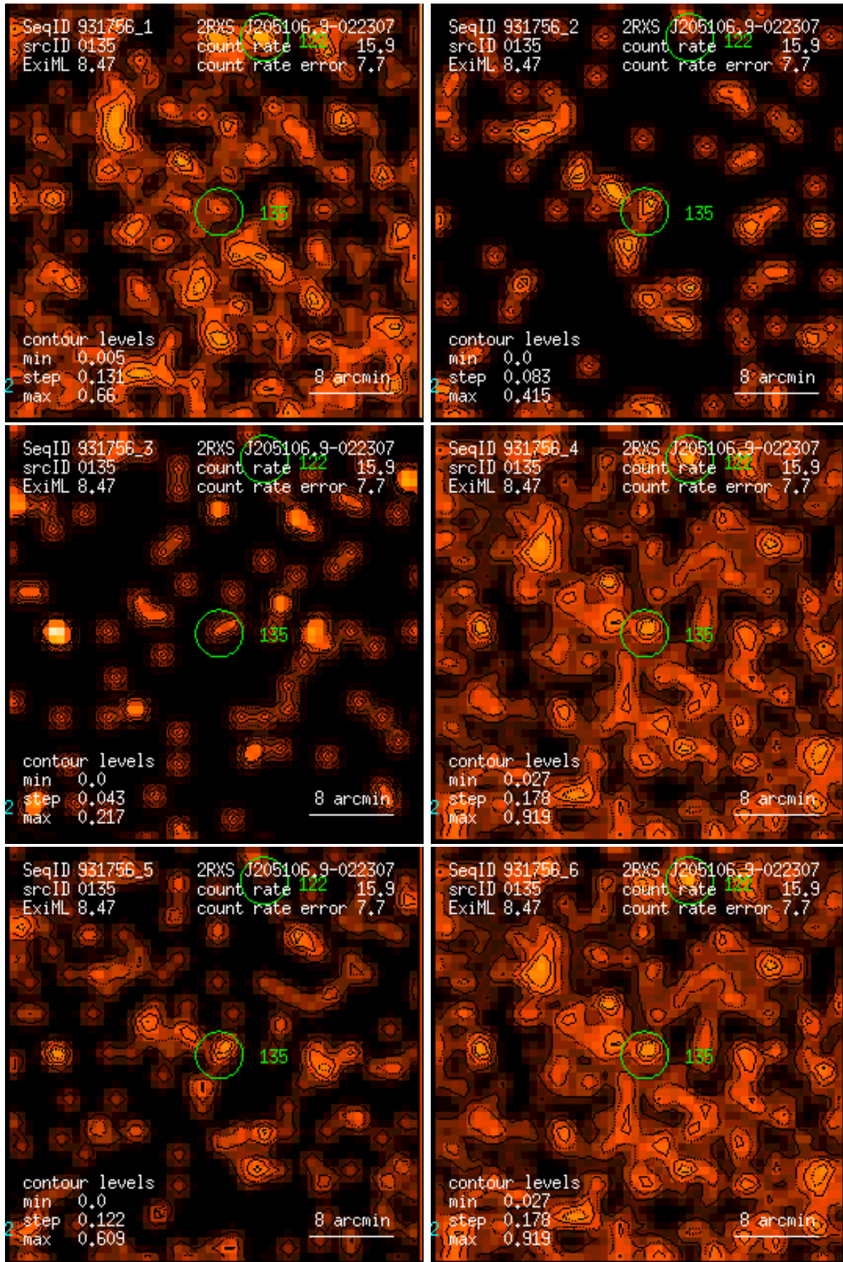
Figure 135: RASS 931756: detection 0135: band rate images, Gaussian filter: (1) PSPC channels 11 – 41, (2) 52 – 90, (3) 91 – 201, (4) 11 – 235, (5) 52 – 201, (6) 11 – 201. Broad band rates in counts/ks. Band rate contour levels in counts/ks/arcmin 2 .
