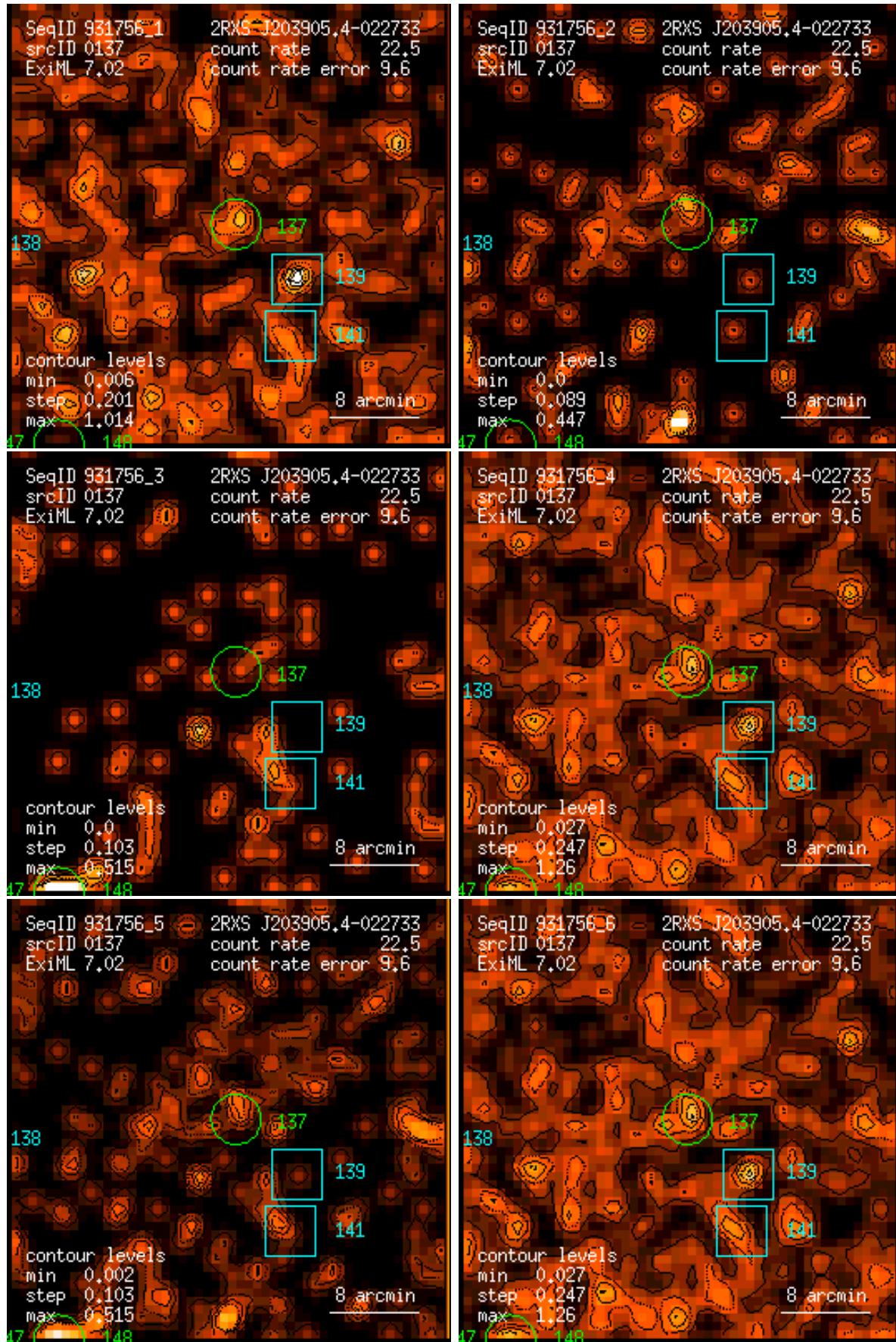
Figure 137: RASS 931756: detection 0137: band rate images, Gaussian filter: (1) PSPC channels 11 – 41, (2) 52 – 90, (3) 91 – 201, (4) 11 – 235, (5) 52 – 201, (6) 11 – 201. Broad band rates in counts/ks. Band rate contour levels in counts/ks/arcmin 2 .
