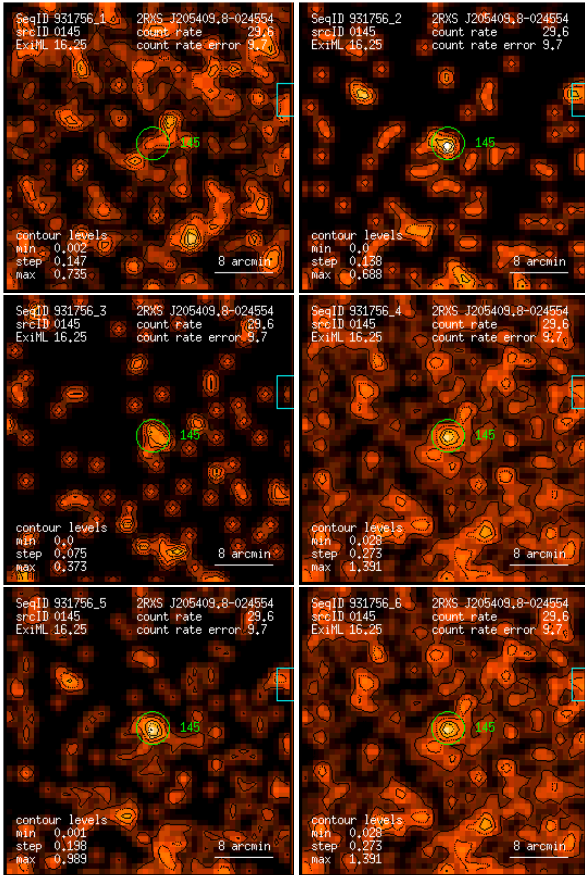
Figure 145: RASS 931756: detection 0145: band rate images, Gaussian filter: (1) PSPC channels 11 – 41, (2) 52 – 90, (3) 91 – 201, (4) 11 – 235, (5) 52 – 201, (6) 11 – 201. Broad band rates in counts/ks. Band rate contour levels in counts/ks/arcmin 2 .
