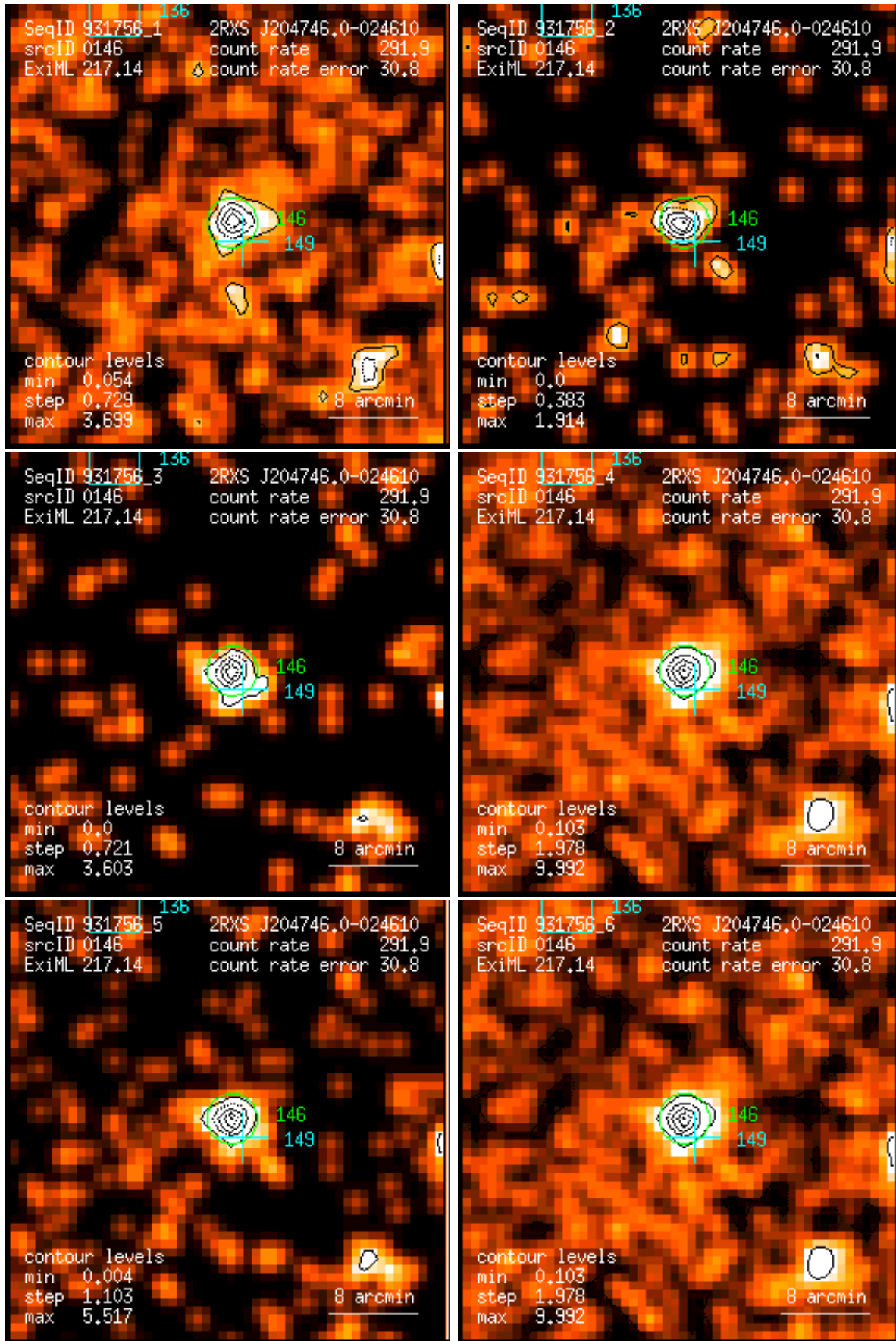
Figure 146: RASS 931756: detection 0146: band rate images, Gaussian filter: (1) PSPC channels 11 – 41, (2) 52 – 90, (3) 91 – 201, (4) 11 – 235, (5) 52 – 201, (6) 11 – 201. Broad band rates in counts/ks. Band rate contour levels in counts/ks/arcmin 2 .
