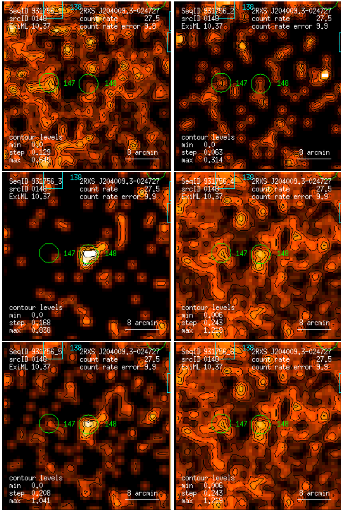
Figure 148: RASS 931756: detection 0148: band rate images, Gaussian filter: (1) PSPC channels 11 – 41, (2) 52 – 90, (3) 91 – 201, (4) 11 – 235, (5) 52 – 201, (6) 11 – 201. Broad band rates in counts/ks. Band rate contour levels in counts/ks/arcmin 2 .
