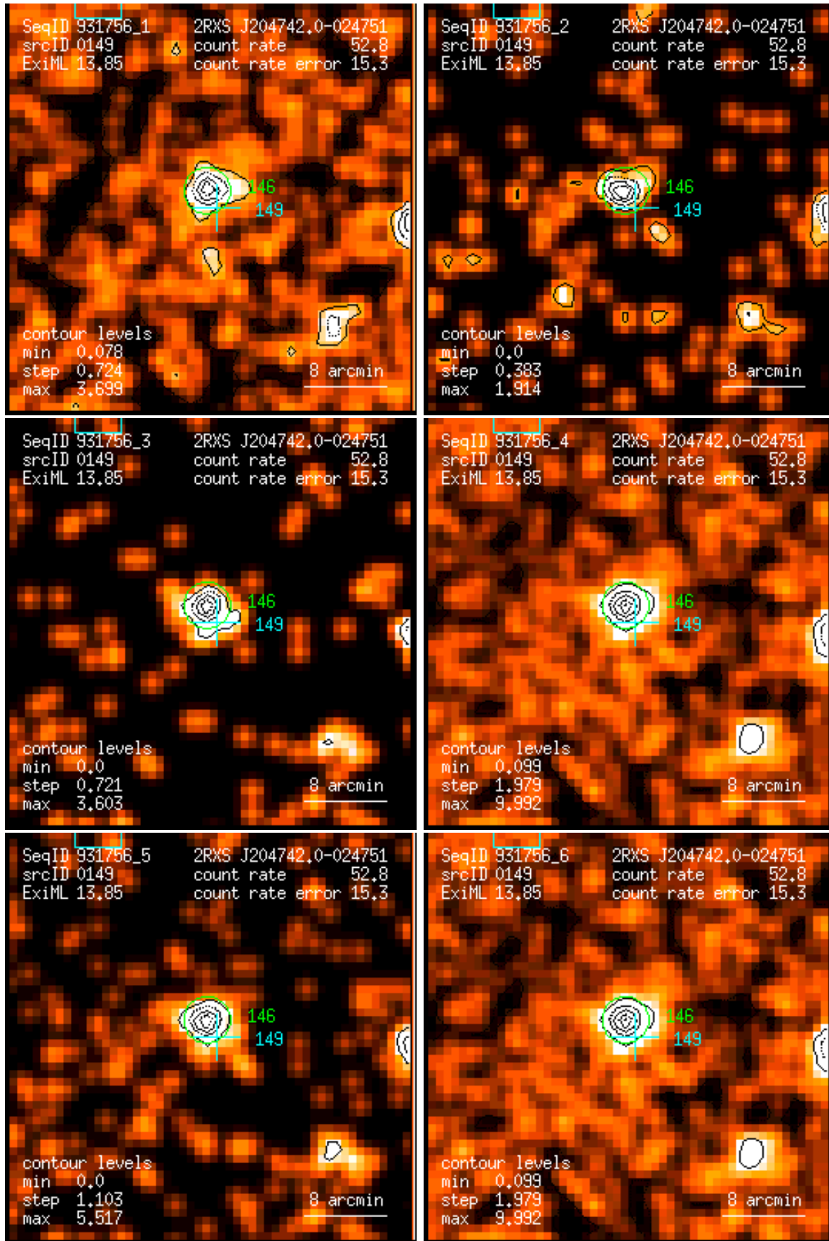
Figure 149: RASS 931756: detection 0149: band rate images, Gaussian filter: (1) PSPC channels 11 – 41, (2) 52 – 90, (3) 91 – 201, (4) 11 – 235, (5) 52 – 201, (6) 11 – 201. Broad band rates in counts/ks. Band rate contour levels in counts/ks/arcmin 2 .
