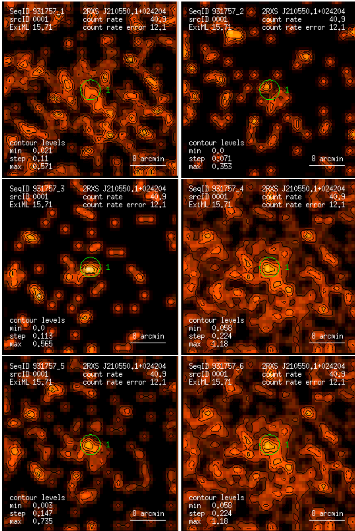
Figure 1: RASS 931757: detection 0001: band rate images, Gaussian filter: (1) PSPC channels 11 – 41, (2) 52 – 90, (3) 91 – 201, (4) 11 – 235, (5) 52 – 201, (6) 11 – 201. Broad band rates in counts/ks. Band rate contour levels in counts/ks/arcmin 2 .
