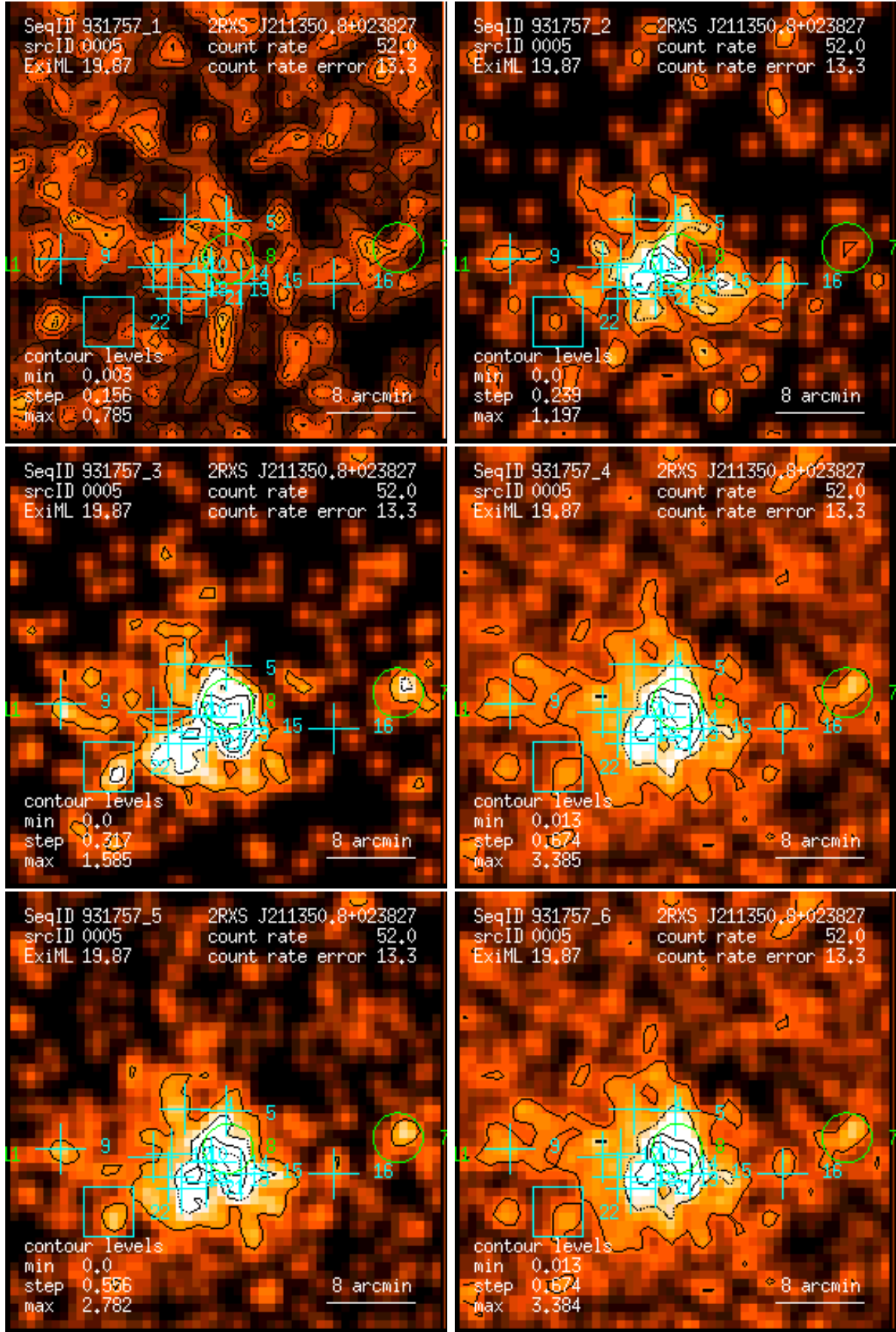
Figure 5: RASS 931757: detection 0005: band rate images, Gaussian filter: (1) PSPC channels 11 – 41, (2) 52 – 90, (3) 91 – 201, (4) 11 – 235, (5) 52 – 201, (6) 11 – 201. Broad band rates in counts/ks. Band rate contour levels in counts/ks/arcmin 2 .
