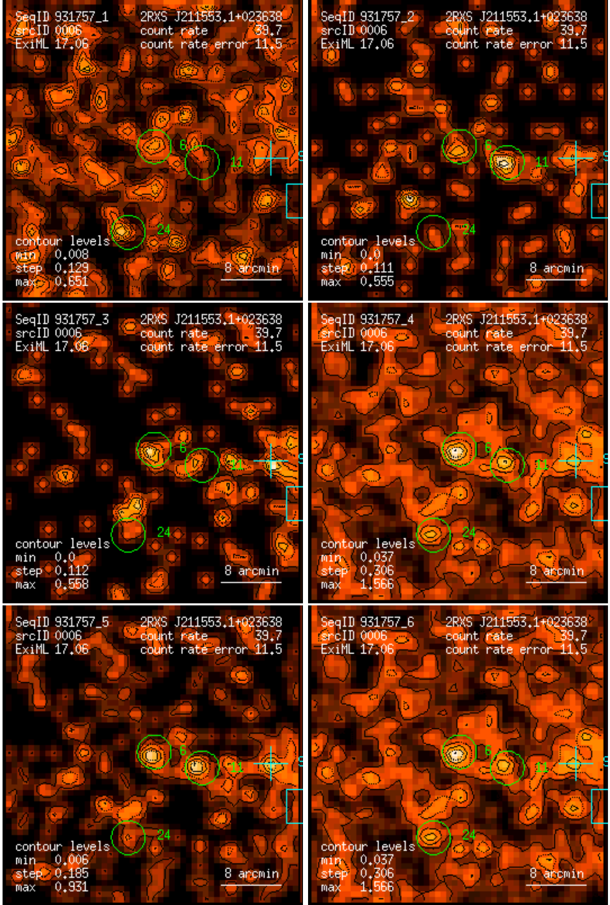
Figure 6: RASS 931757: detection 0006: band rate images, Gaussian filter: (1) PSPC channels 11 – 41, (2) 52 – 90, (3) 91 – 201, (4) 11 – 235, (5) 52 – 201, (6) 11 – 201. Broad band rates in counts/ks. Band rate contour levels in counts/ks/arcmin 2 .
