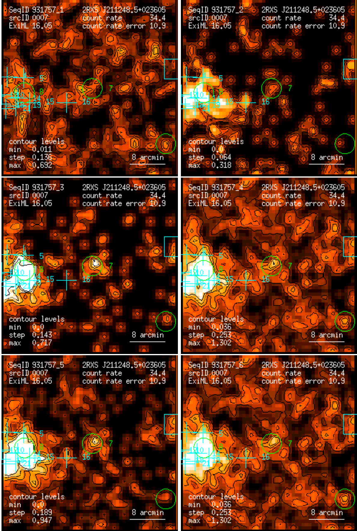
Figure 7: RASS 931757: detection 0007: band rate images, Gaussian filter: (1) PSPC channels 11 – 41, (2) 52 – 90, (3) 91 – 201, (4) 11 – 235, (5) 52 – 201, (6) 11 – 201. Broad band rates in counts/ks. Band rate contour levels in counts/ks/arcmin 2 .
