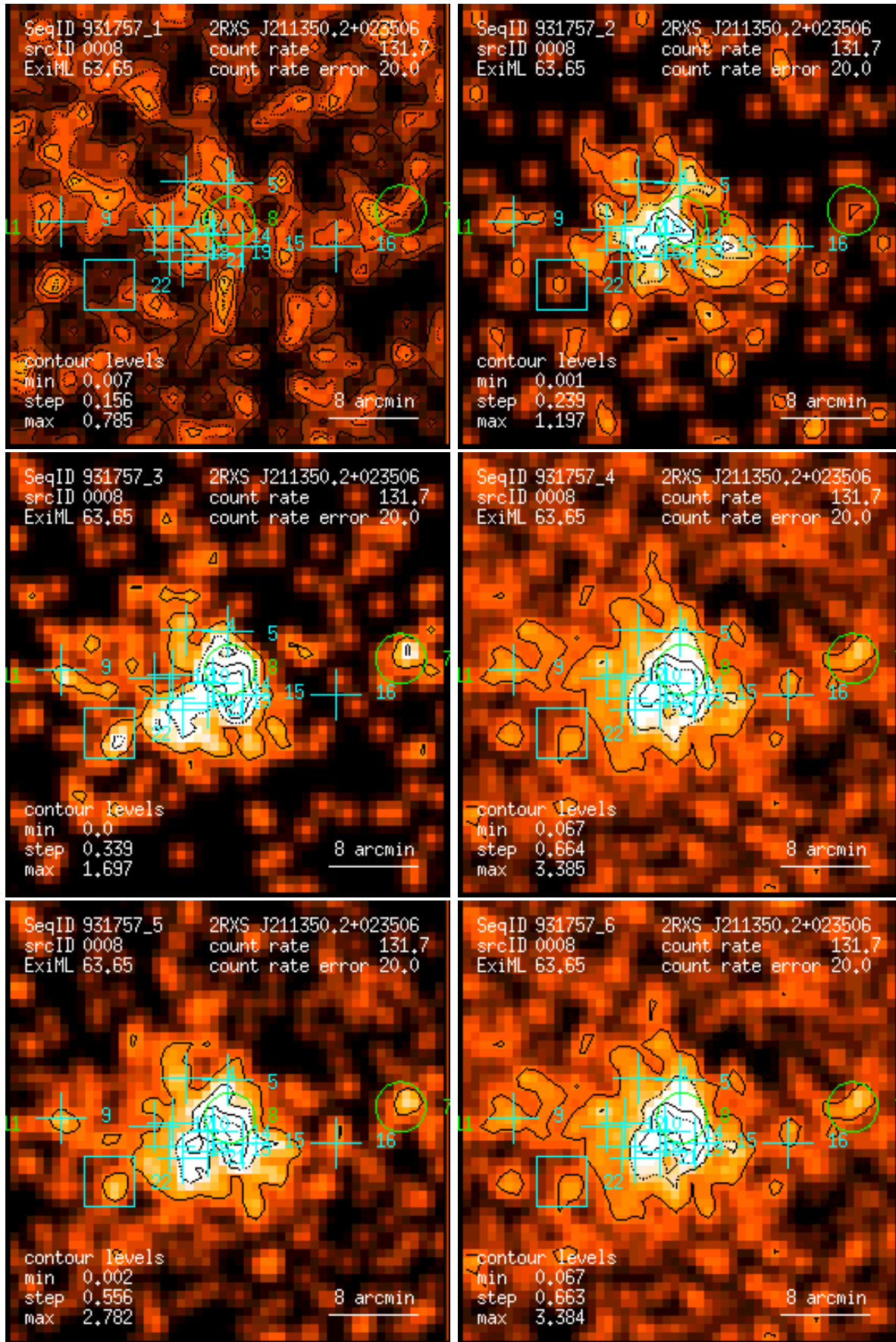
Figure 8: RASS 931757: detection 0008: band rate images, Gaussian filter: (1) PSPC channels 11 – 41, (2) 52 – 90, (3) 91 – 201, (4) 11 – 235, (5) 52 – 201, (6) 11 – 201. Broad band rates in counts/ks. Band rate contour levels in counts/ks/arcmin 2 .
