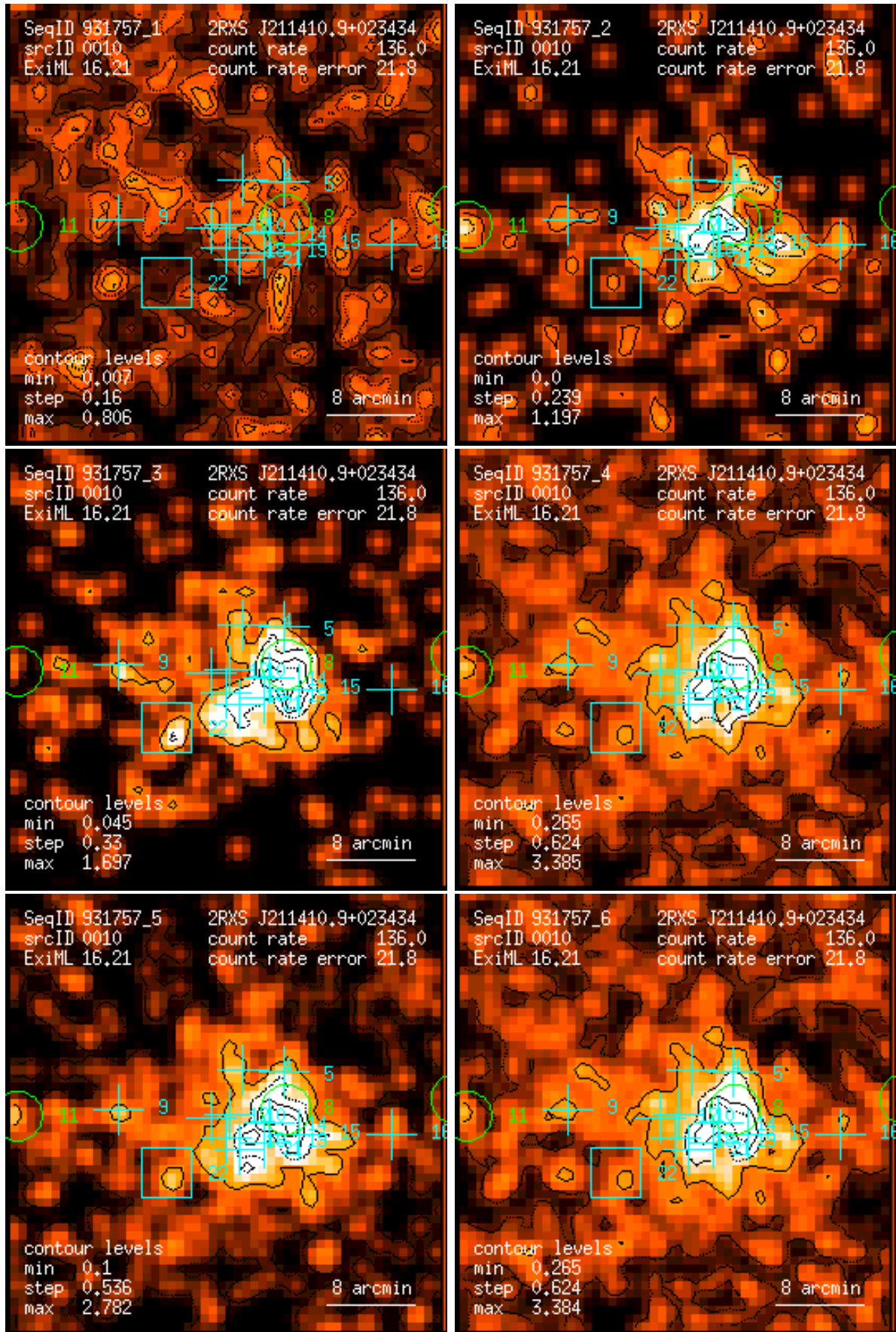
Figure 10: RASS 931757: detection 0010: band rate images, Gaussian filter: (1) PSPC channels 11 – 41, (2) 52 – 90, (3) 91 – 201, (4) 11 – 235, (5) 52 – 201, (6) 11 – 201. Broad band rates in counts/ks. Band rate contour levels in counts/ks/arcmin 2 .
