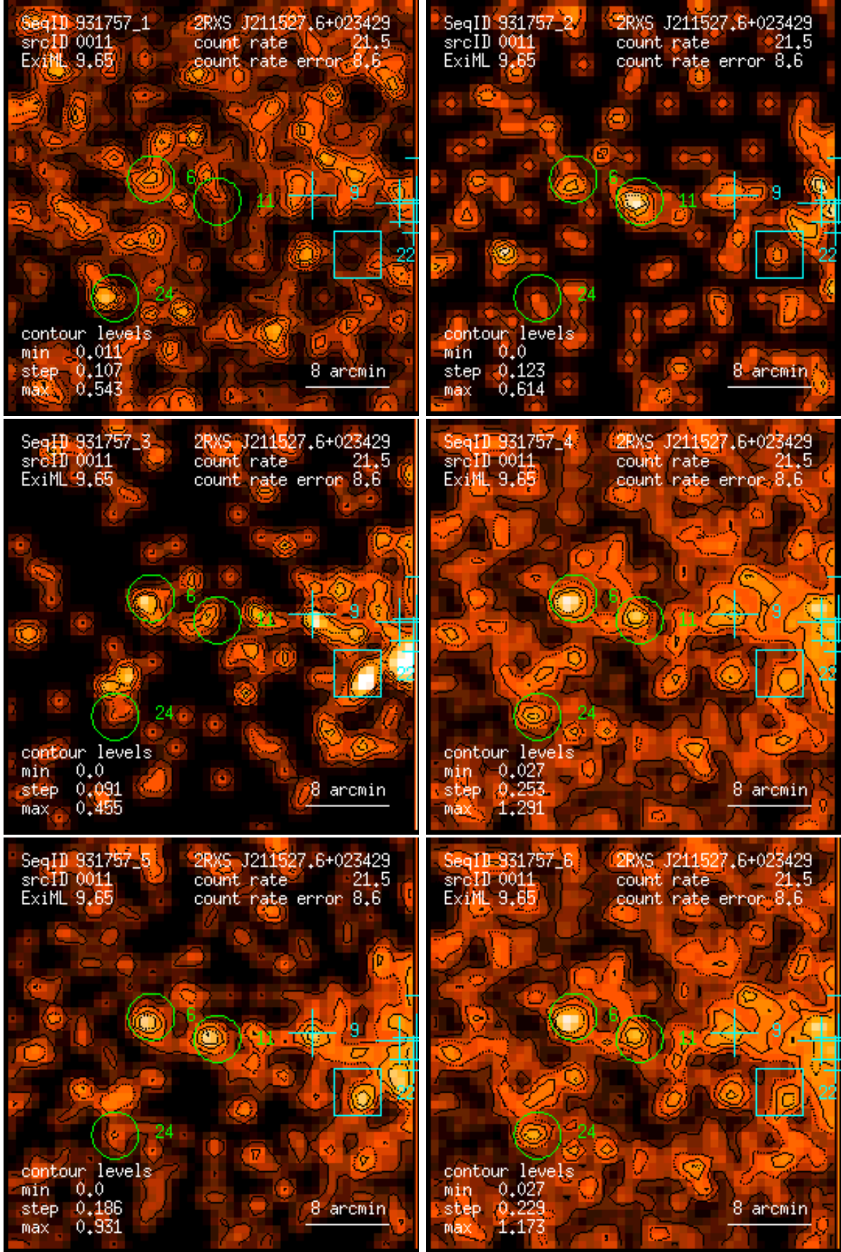
Figure 11: RASS 931757: detection 0011: band rate images, Gaussian filter: (1) PSPC channels 11 – 41, (2) 52 – 90, (3) 91 – 201, (4) 11 – 235, (5) 52 – 201, (6) 11 – 201. Broad band rates in counts/ks. Band rate contour levels in counts/ks/arcmin 2 .
