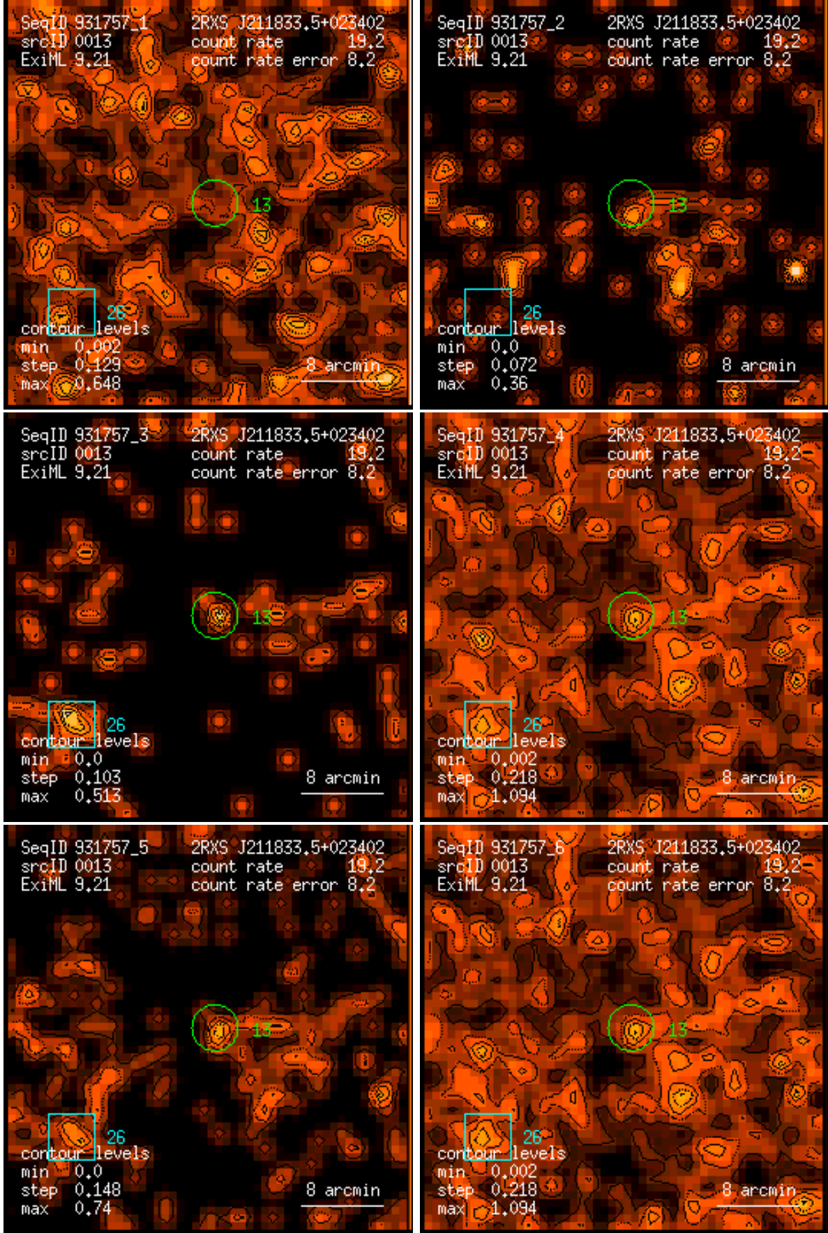
Figure 13: RASS 931757: detection 0013: band rate images, Gaussian filter: (1) PSPC channels 11 – 41, (2) 52 – 90, (3) 91 – 201, (4) 11 – 235, (5) 52 – 201, (6) 11 – 201. Broad band rates in counts/ks. Band rate contour levels in counts/ks/arcmin 2 .
