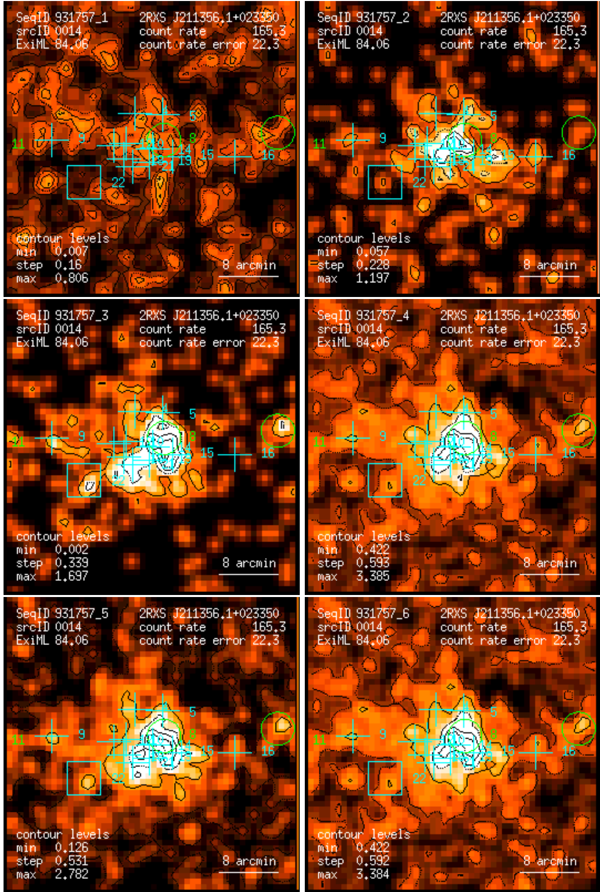
Figure 14: RASS 931757: detection 0014: band rate images, Gaussian filter: (1) PSPC channels 11 – 41, (2) 52 – 90, (3) 91 – 201, (4) 11 – 235, (5) 52 – 201, (6) 11 – 201. Broad band rates in counts/ks. Band rate contour levels in counts/ks/arcmin 2 .
