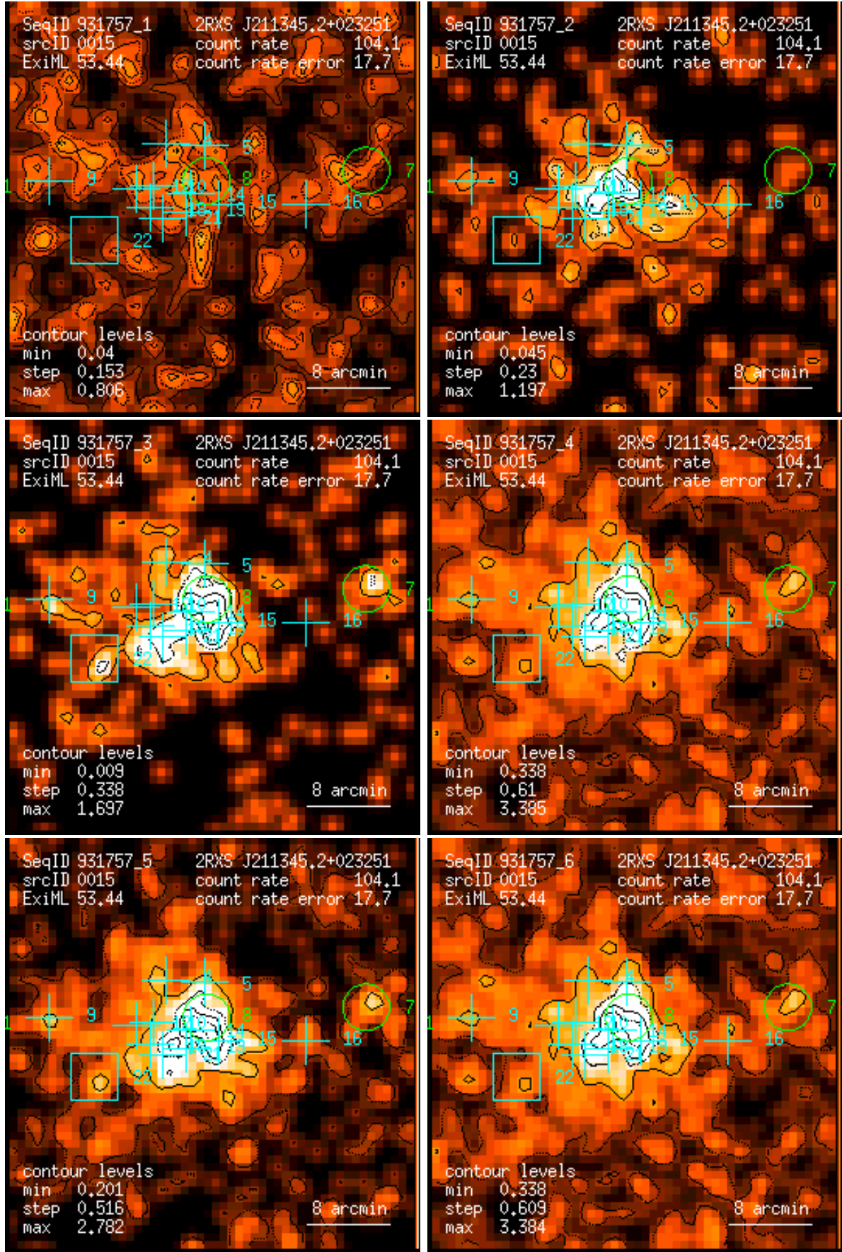
Figure 15: RASS 931757: detection 0015: band rate images, Gaussian filter: (1) PSPC channels 11 – 41, (2) 52 – 90, (3) 91 – 201, (4) 11 – 235, (5) 52 – 201, (6) 11 – 201. Broad band rates in counts/ks. Band rate contour levels in counts/ks/arcmin 2 .
