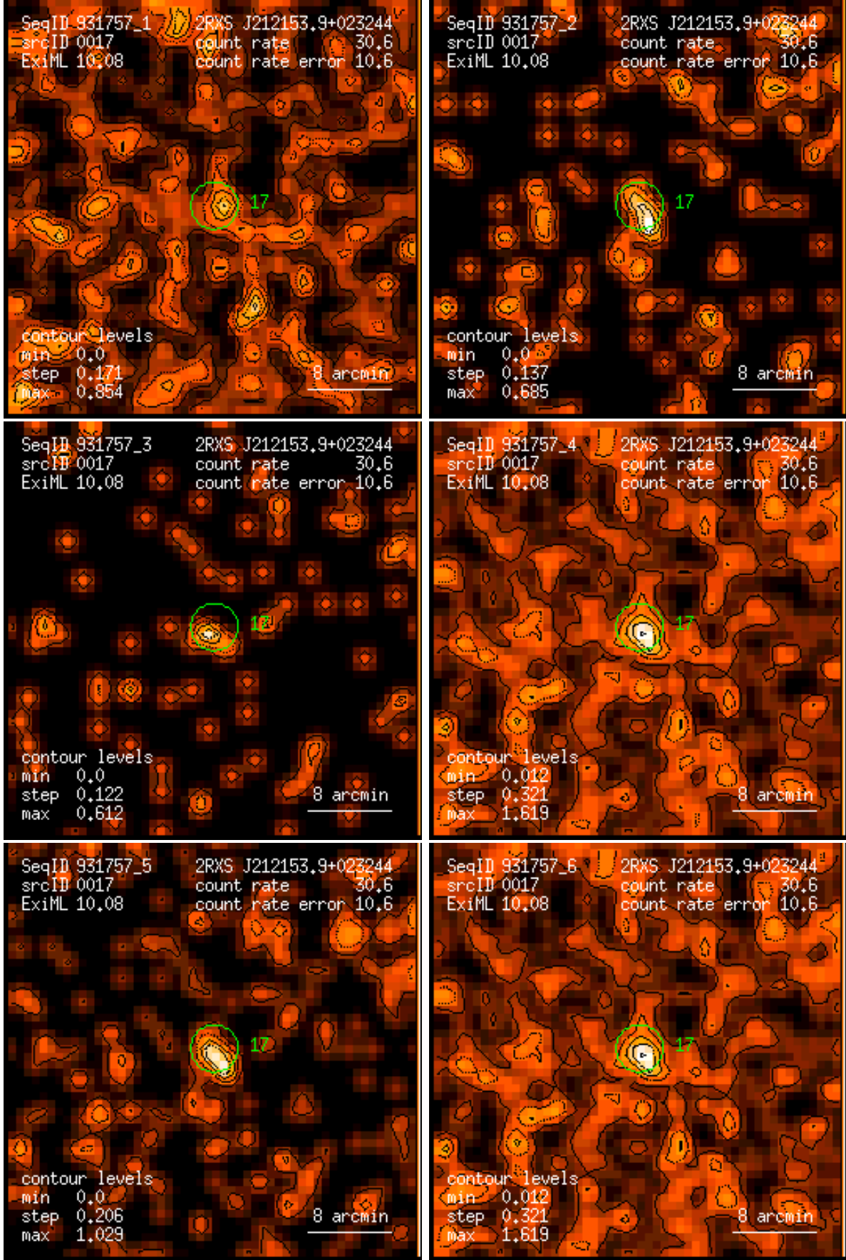
Figure 17: RASS 931757: detection 0017: band rate images, Gaussian filter: (1) PSPC channels 11 – 41, (2) 52 – 90, (3) 91 – 201, (4) 11 – 235, (5) 52 – 201, (6) 11 – 201. Broad band rates in counts/ks. Band rate contour levels in counts/ks/arcmin 2 .
