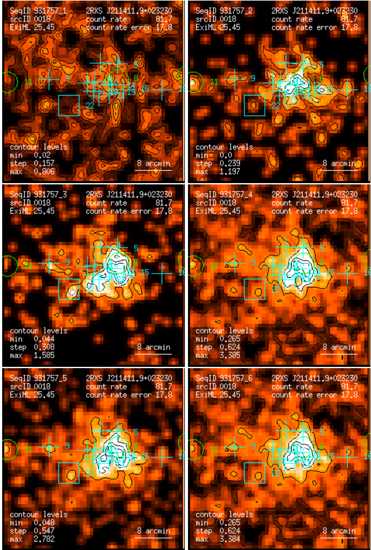
Figure 18: RASS 931757: detection 0018: band rate images, Gaussian filter: (1) PSPC channels 11 – 41, (2) 52 – 90, (3) 91 – 201, (4) 11 – 235, (5) 52 – 201, (6) 11 – 201. Broad band rates in counts/ks. Band rate contour levels in counts/ks/arcmin 2 .
