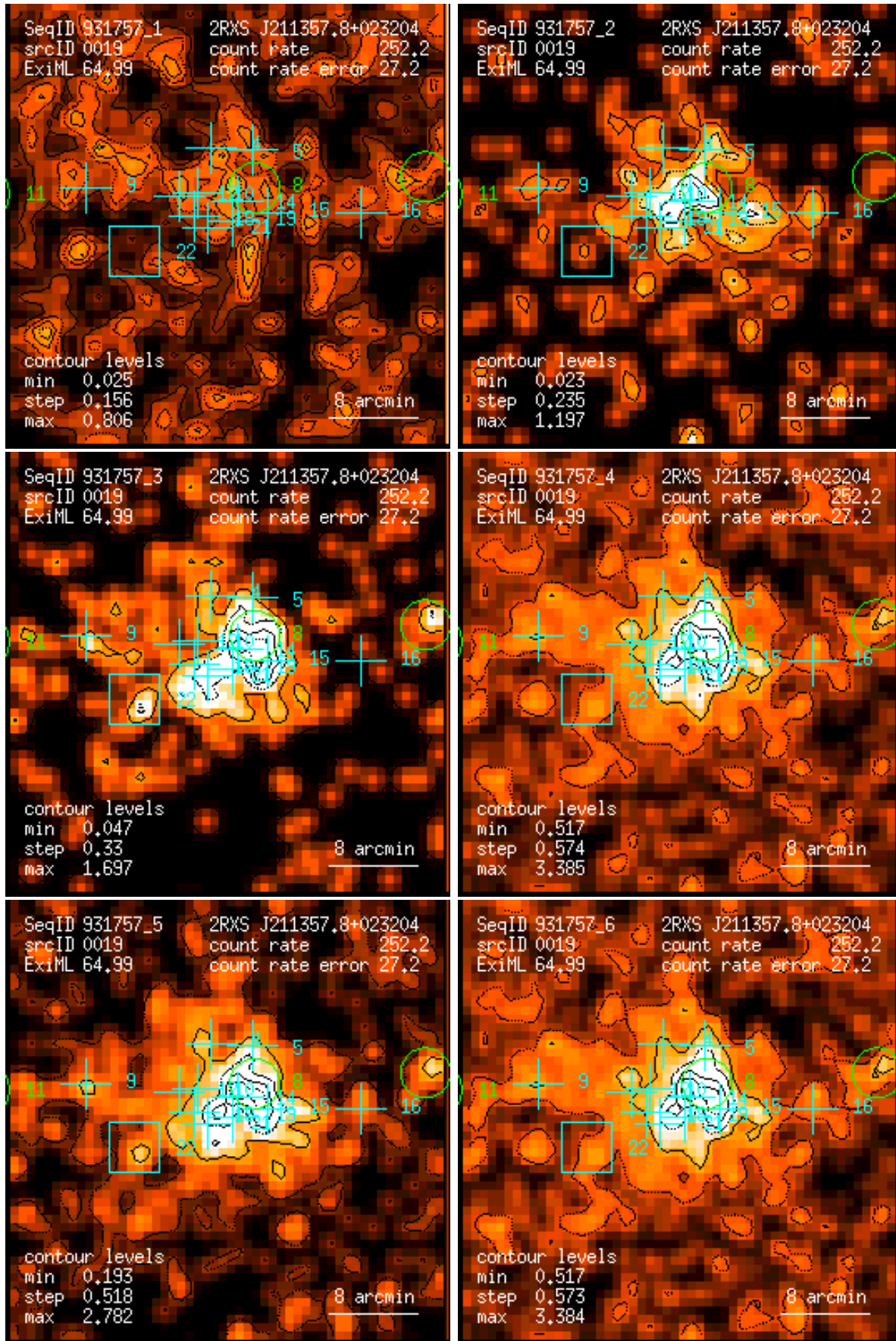
Figure 19: RASS 931757: detection 0019: band rate images, Gaussian filter: (1) PSPC channels 11 – 41, (2) 52 – 90, (3) 91 – 201, (4) 11 – 235, (5) 52 – 201, (6) 11 – 201. Broad band rates in counts/ks. Band rate contour levels in counts/ks/arcmin 2 .
