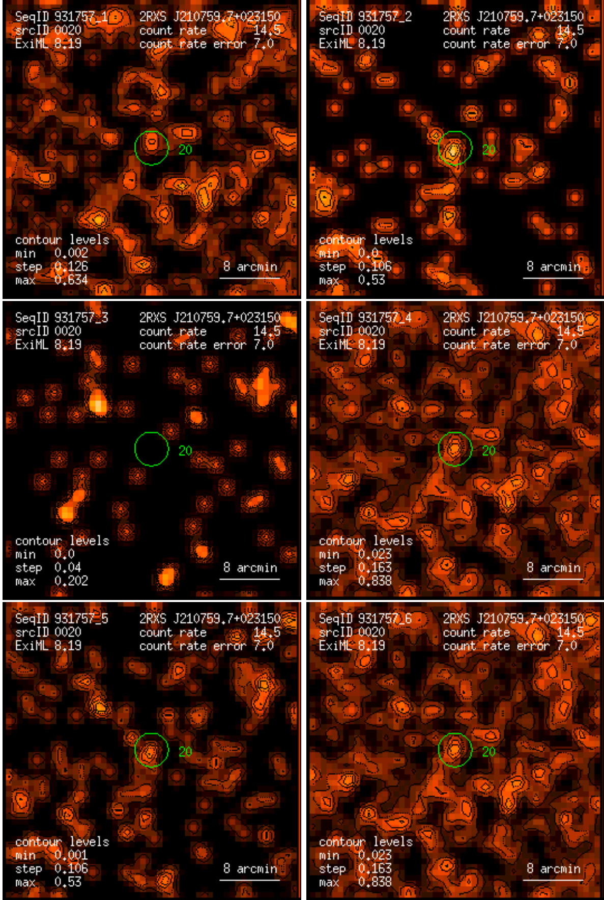
Figure 20: RASS 931757: detection 0020: band rate images, Gaussian filter: (1) PSPC channels 11 – 41, (2) 52 – 90, (3) 91 – 201, (4) 11 – 235, (5) 52 – 201, (6) 11 – 201. Broad band rates in counts/ks. Band rate contour levels in counts/ks/arcmin 2 .
