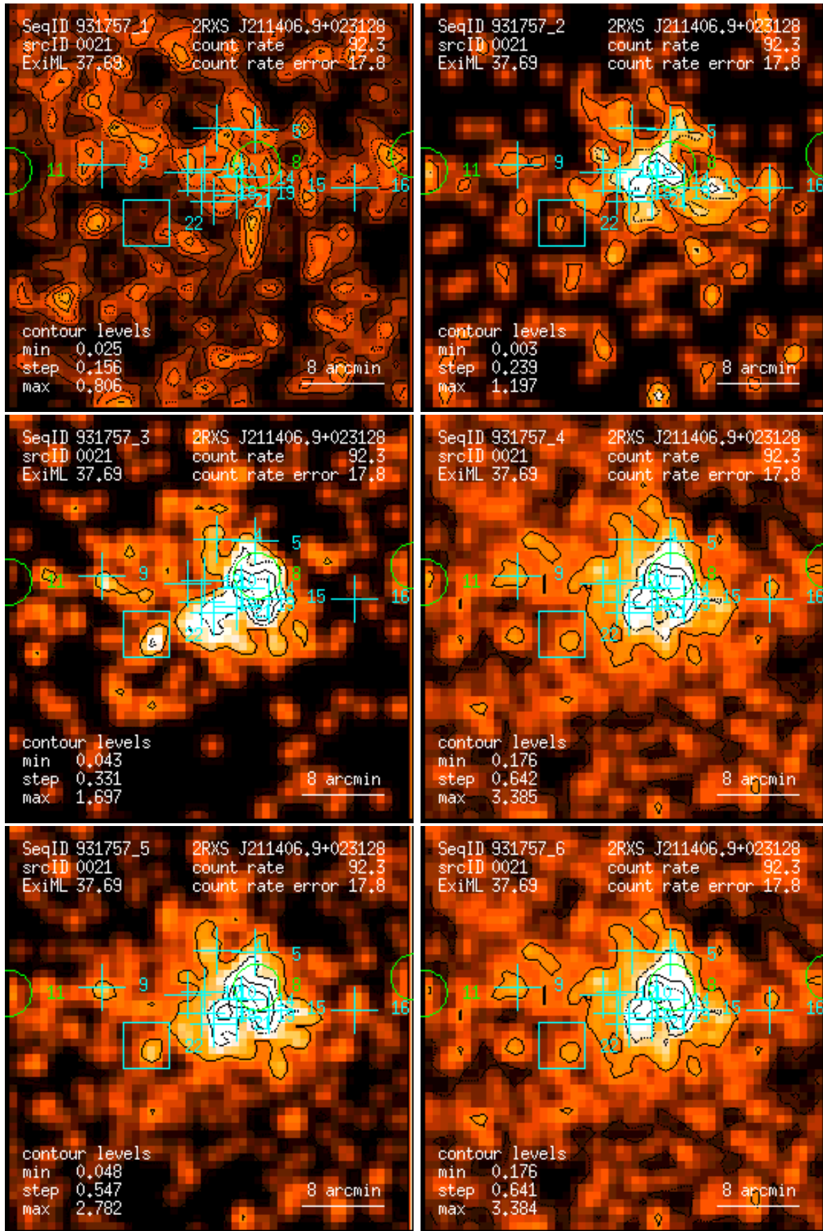
Figure 21: RASS 931757: detection 0021: band rate images, Gaussian filter: (1) PSPC channels 11 – 41, (2) 52 – 90, (3) 91 – 201, (4) 11 – 235, (5) 52 – 201, (6) 11 – 201. Broad band rates in counts/ks. Band rate contour levels in counts/ks/arcmin 2 .
