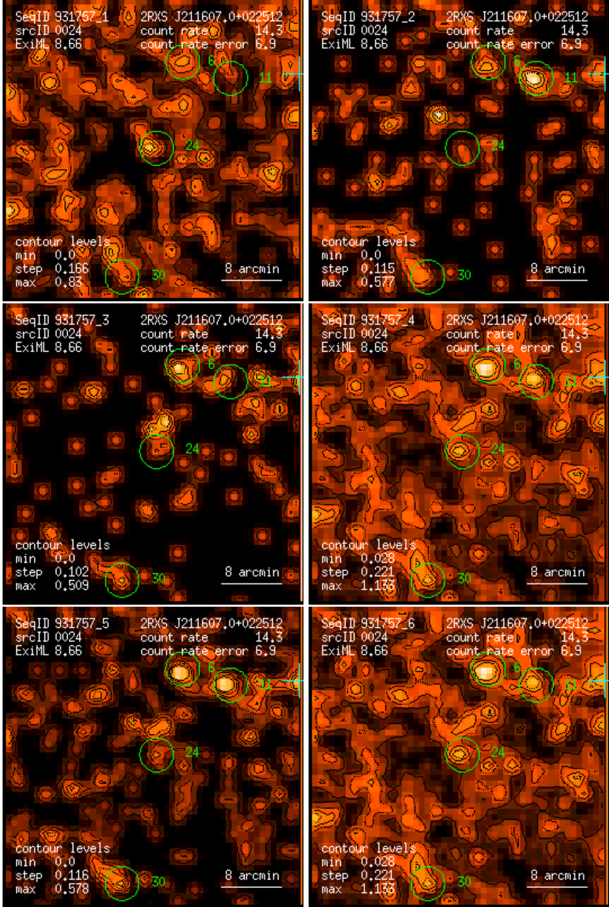
Figure 24: RASS 931757: detection 0024: band rate images, Gaussian filter: (1) PSPC channels 11 – 41, (2) 52 – 90, (3) 91 – 201, (4) 11 – 235, (5) 52 – 201, (6) 11 – 201. Broad band rates in counts/ks. Band rate contour levels in counts/ks/arcmin 2 .
