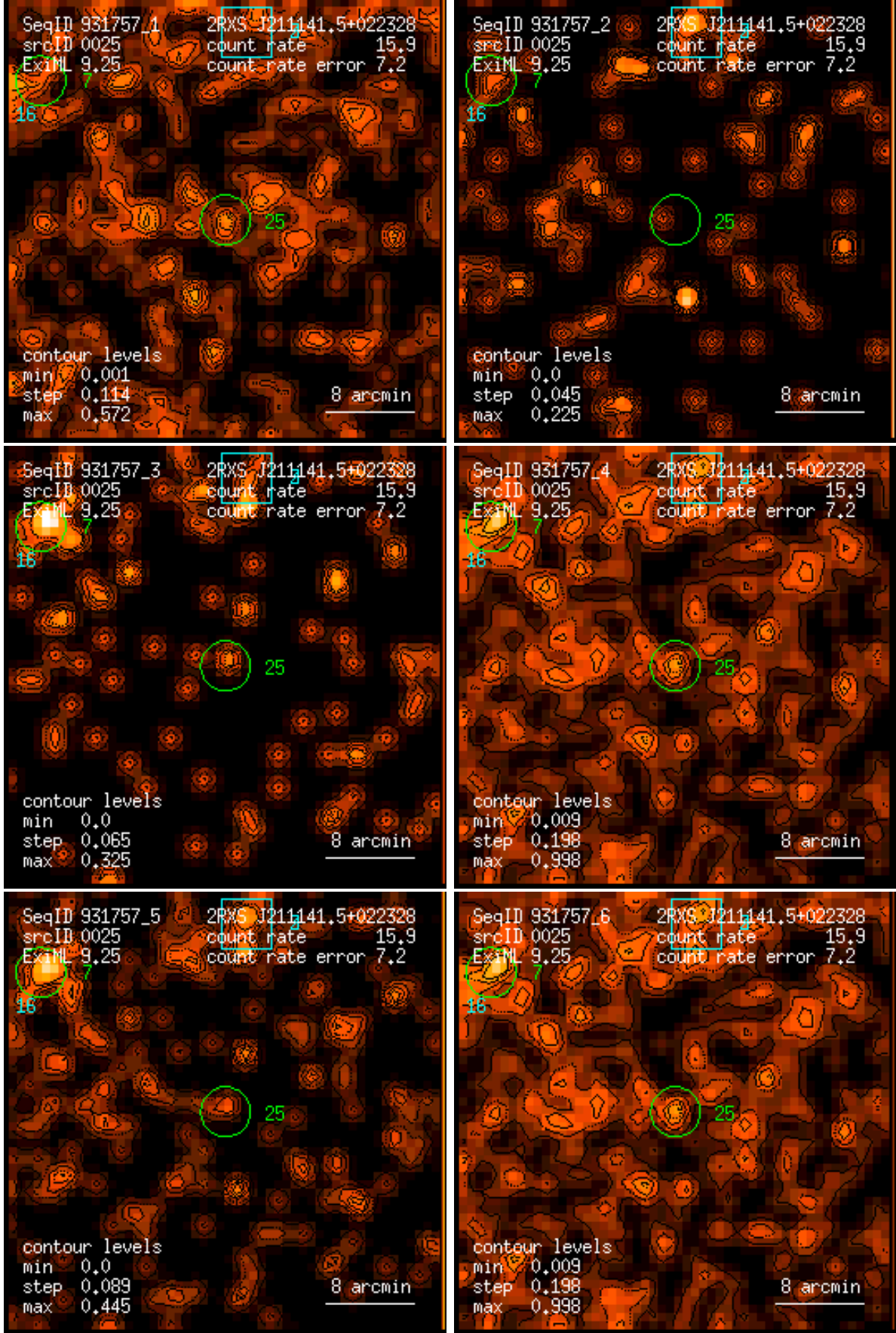
Figure 25: RASS 931757: detection 0025: band rate images, Gaussian filter: (1) PSPC channels 11 – 41, (2) 52 – 90, (3) 91 – 201, (4) 11 – 235, (5) 52 – 201, (6) 11 – 201. Broad band rates in counts/ks. Band rate contour levels in counts/ks/arcmin 2 .
